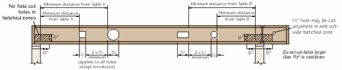
FIGURE 3—ALLOWABLE HOLE SIZE AND LOCATION FOR THE TJI 110, TJI 210, TJI 230, TJI 360 AND TJI 560 JOISTS (TABLES A AND B), AND TJI 100C AND 300C JOISTS (TABLES C AND D)
