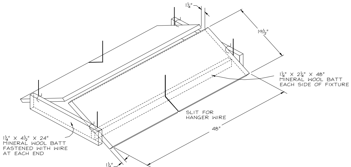
FIGURE 6—LIGHT FIXTURE PROTECTION (See Section 4.17.1, Item 5 for detailed description of mineral wool batts.) For SI: 1 inch = 25.4 mm.
