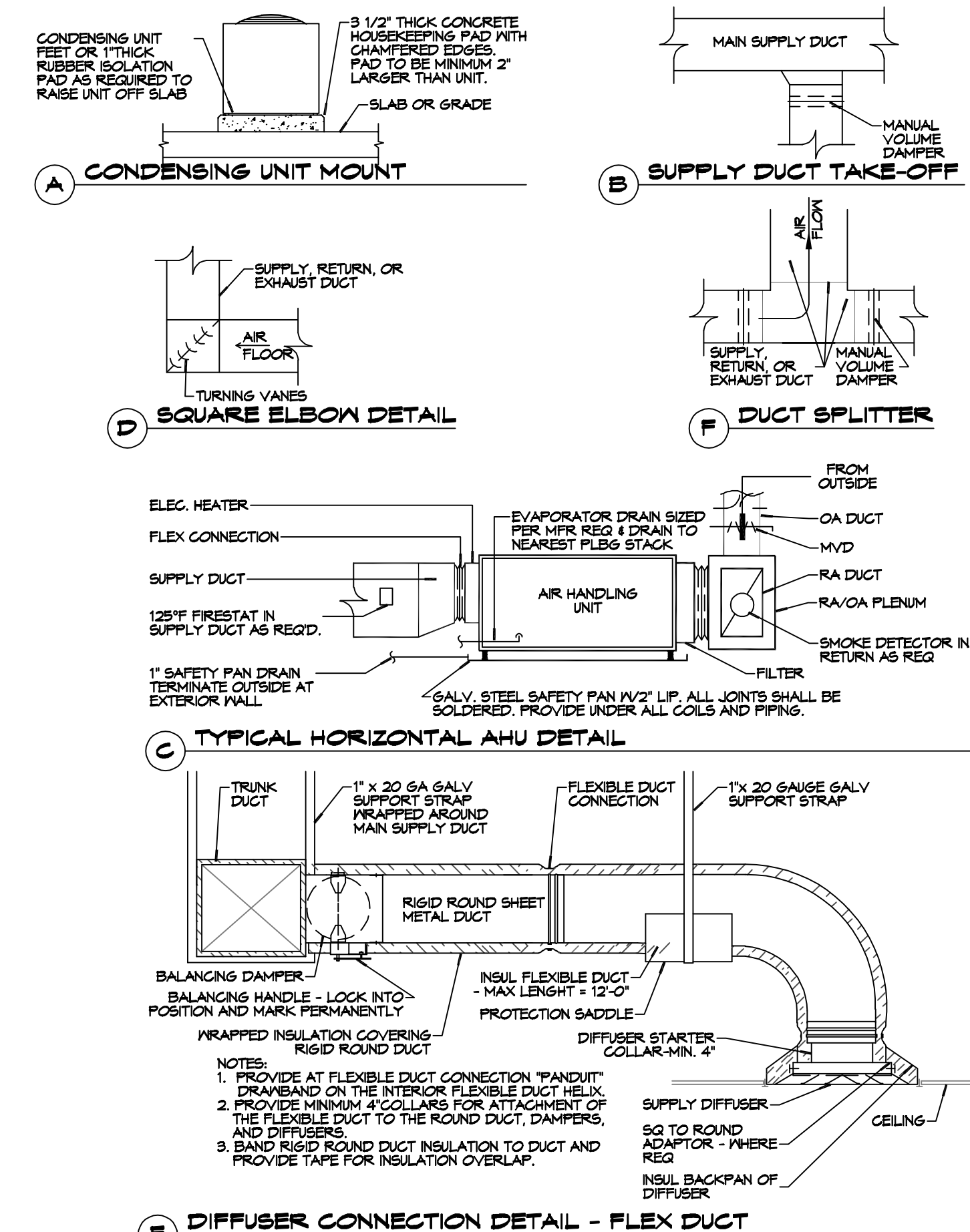
(E) DIFFUSER CONNECTION DETAIL - FLEX DUCT
