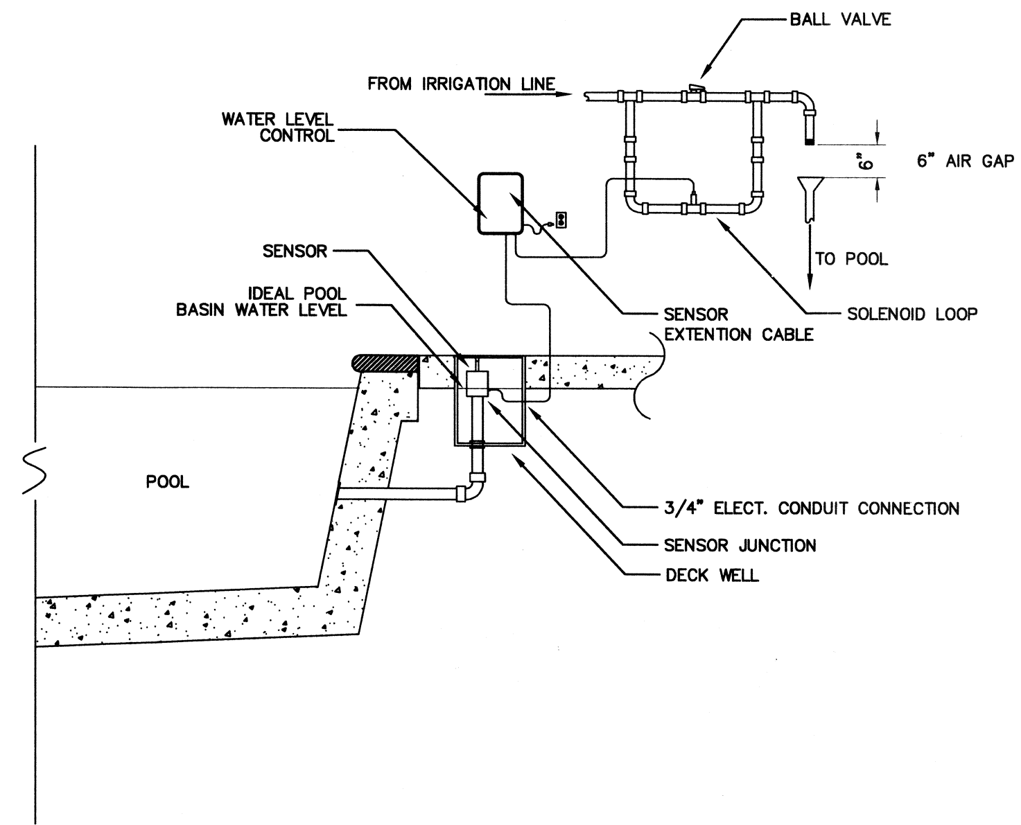
2 WATER LEVEL CONTROLLER PL1.2 SCALE: 1/2" = 1'-0"
