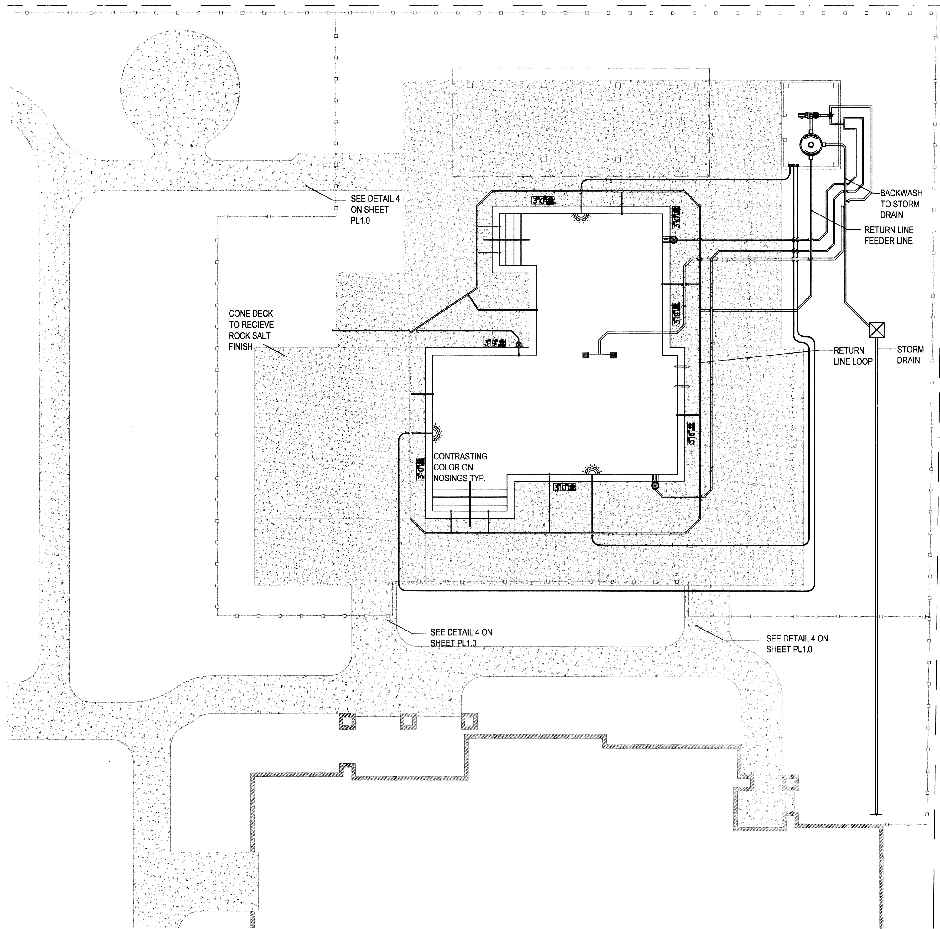
1 POOL PLUMBING PLAN PL1.2 SCALE: 1/8" = 1'-0"
