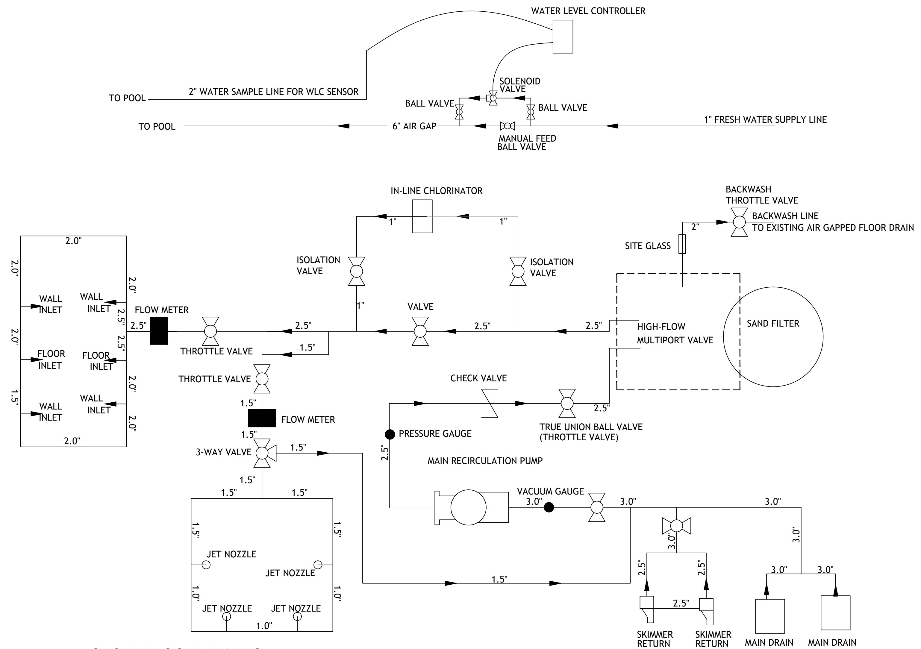
01 SYSTEM SCHEMATIC PL-1.4 SCALE: NOT TO SCALE
