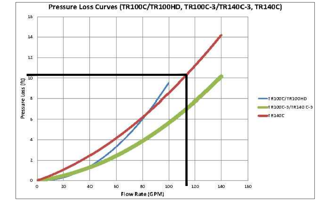
03 SAND FILTER PERFORMANCE CURVE PL-1.4 SCALE: NOT TO SCALE
