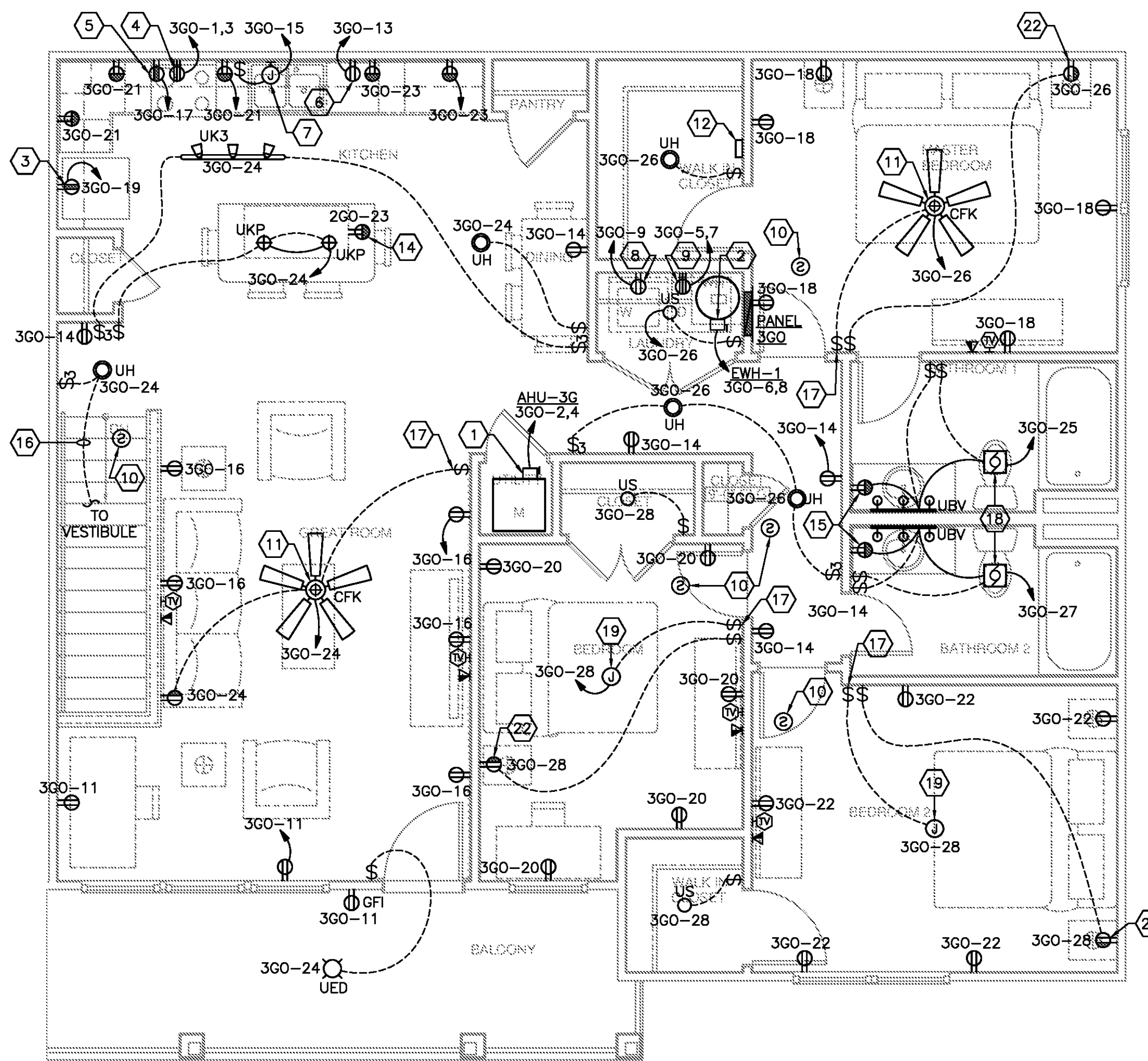
UNIT - 3GO 1/4" = 1'-0"
