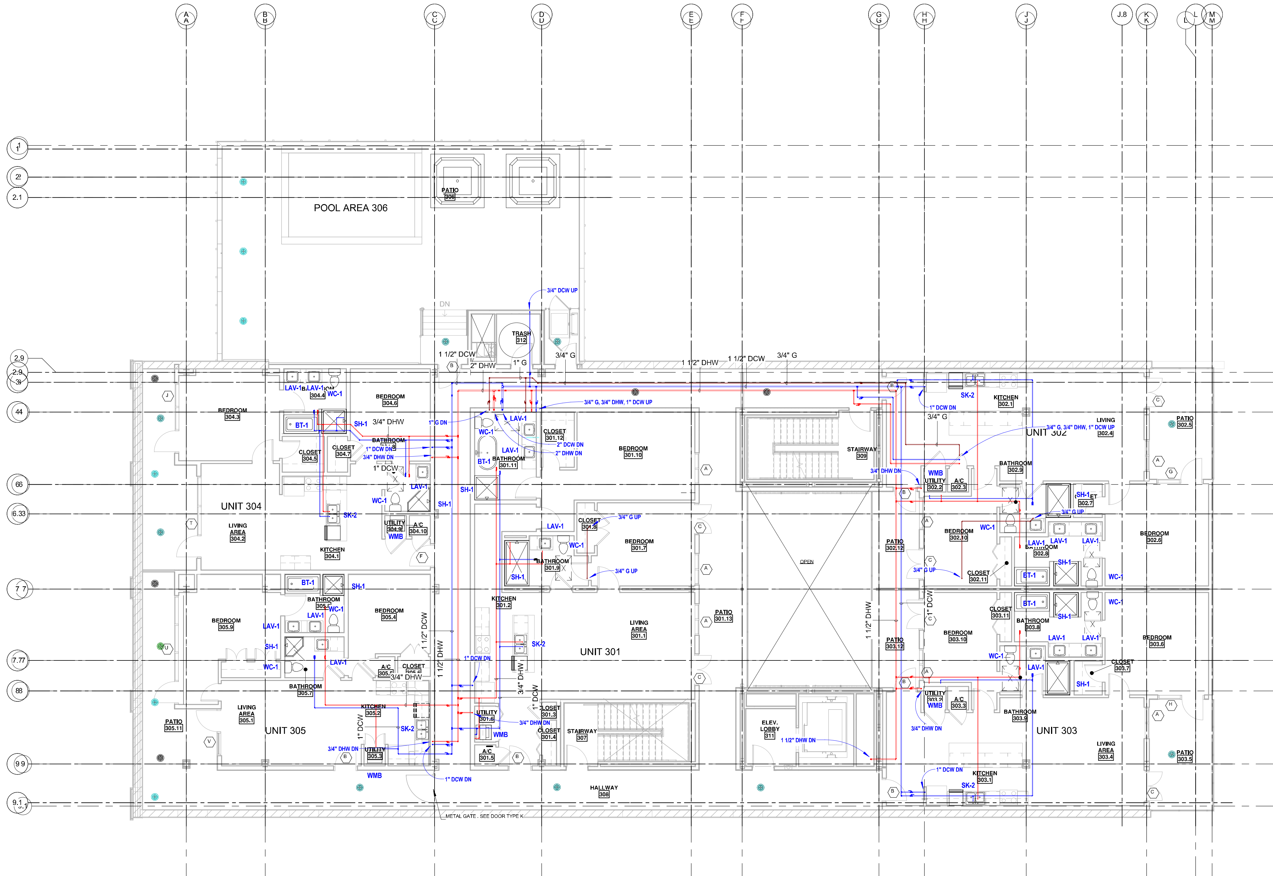
1 3rd FLOOR - PLUMBING - WATER 1/8" = 1'-0"
