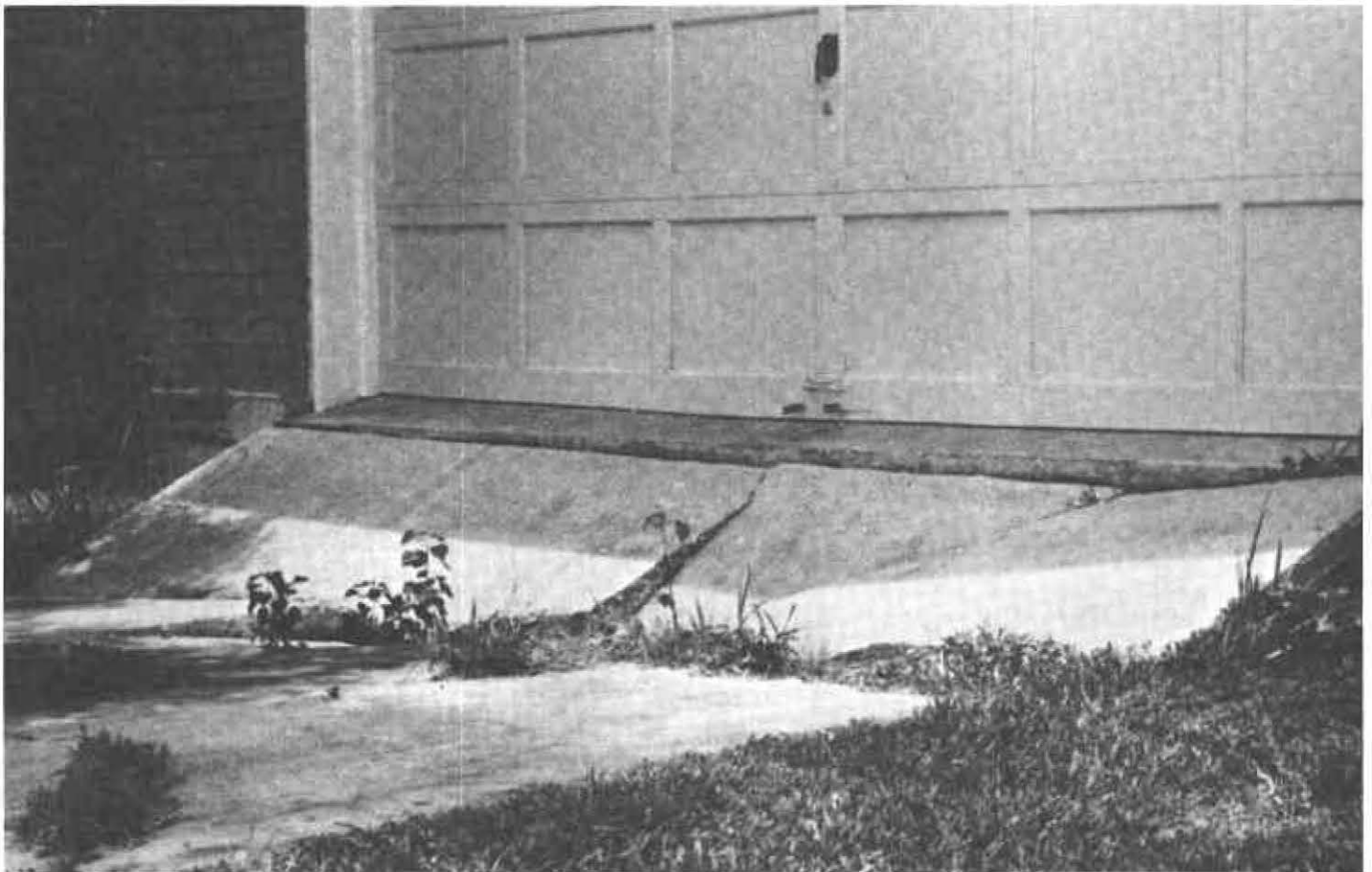
Figure 7.—Subsidence on this Kenner muck, drained, exposes building foundations and causes driveways and sidewalks to warp and crack.
