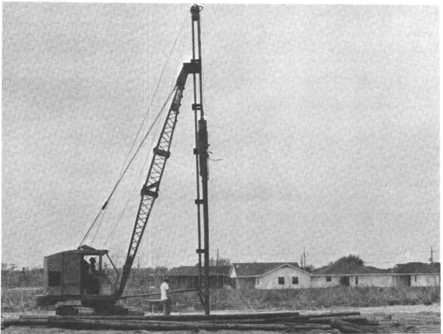
Figure 1.—Wooden pilings, driven deep into the soil, help to provide support for the foundations of houses without basements on Allemands muck, drained.
