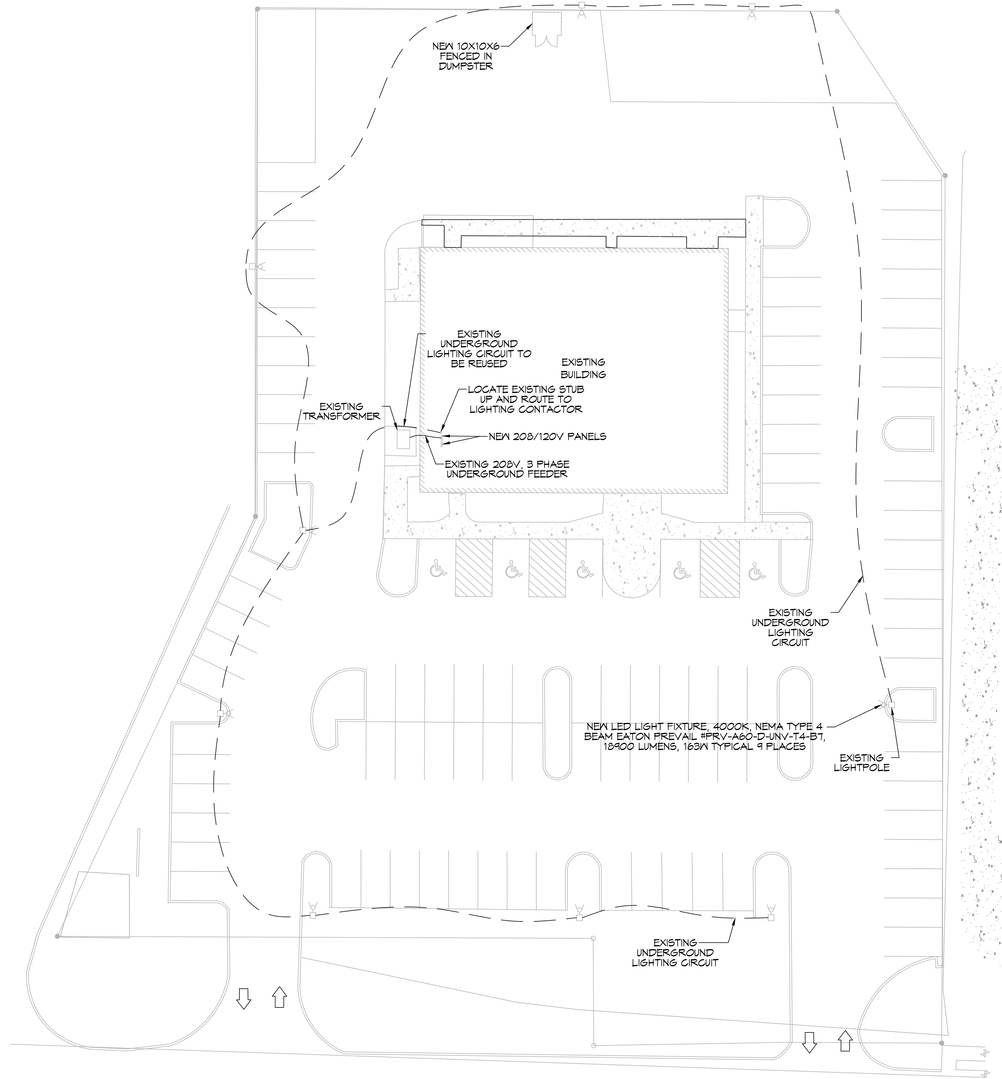
1 SITE LIGHTING PLAN SCALE: 1" = 20'
