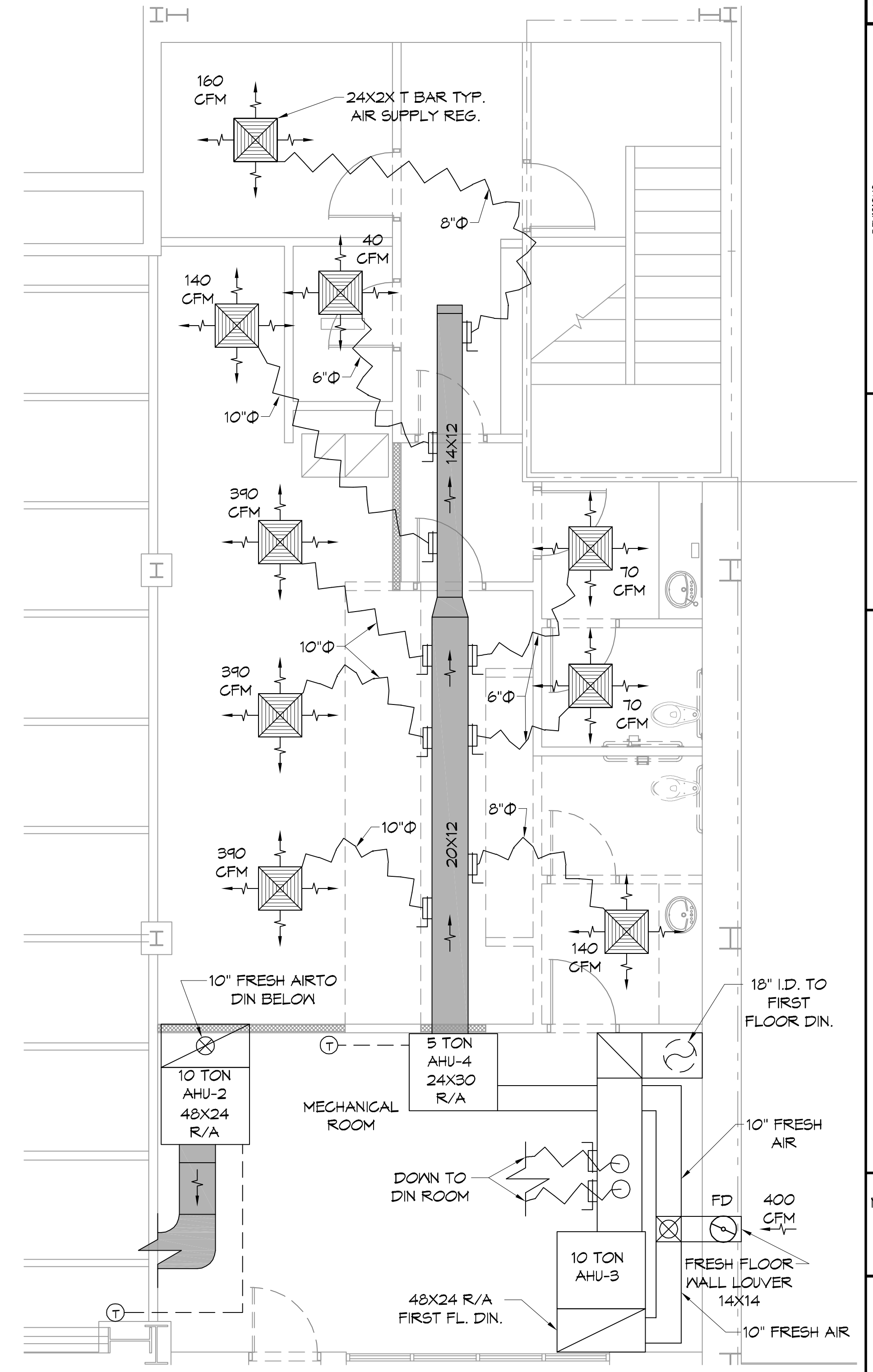
2 MECHANICAL PLAN SECOND FLOOR SCALE: 1/4"=1'-0"
