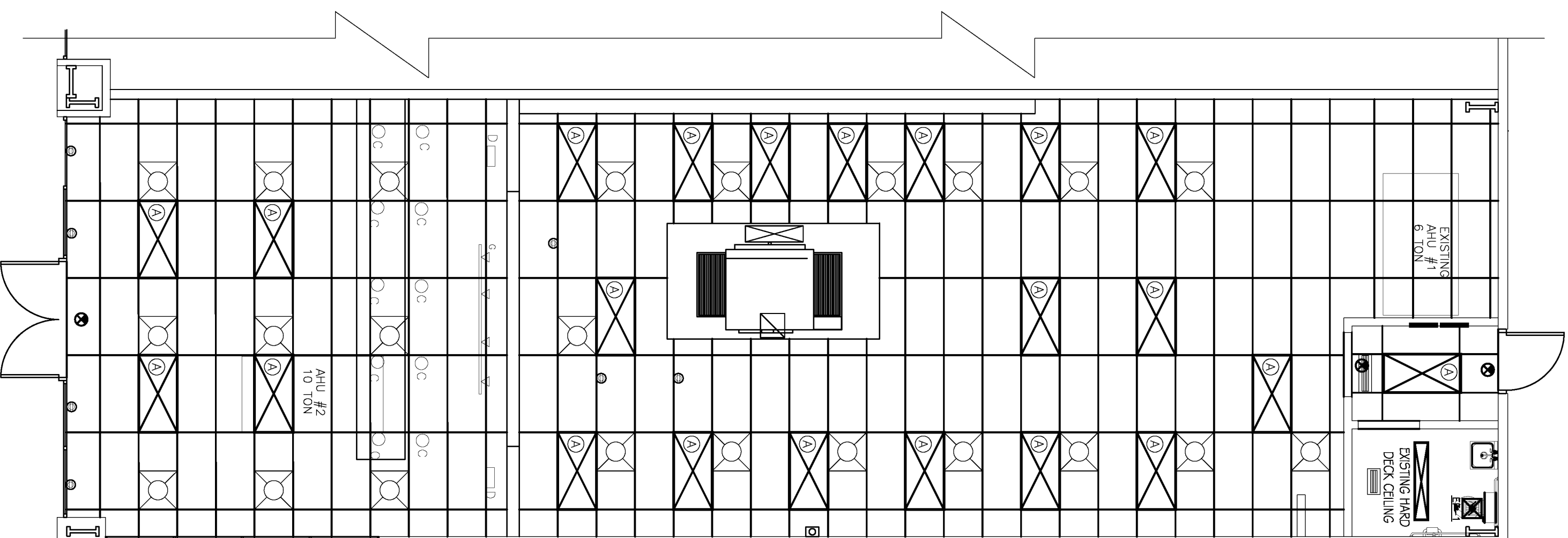
REFLECTED CEILING PLAN SCALE: 3/16" = 1'-0"
