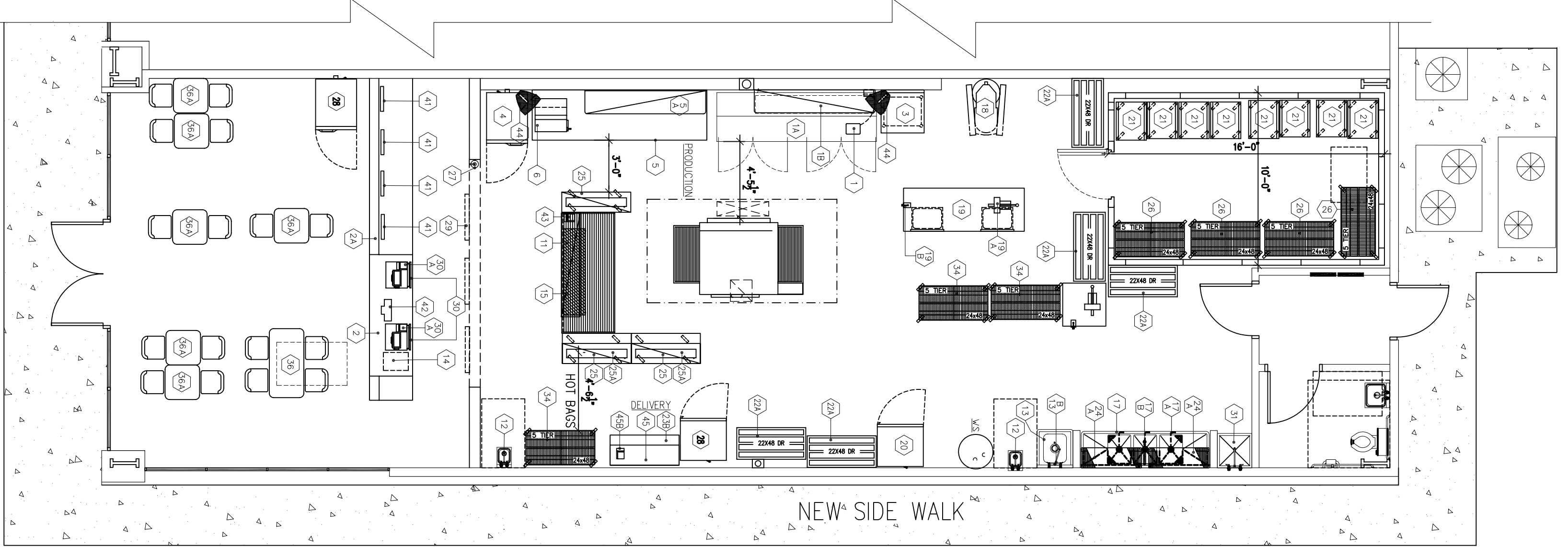
EQUIPMENT PLAN SCALE: 3/8" = 1'-0"
