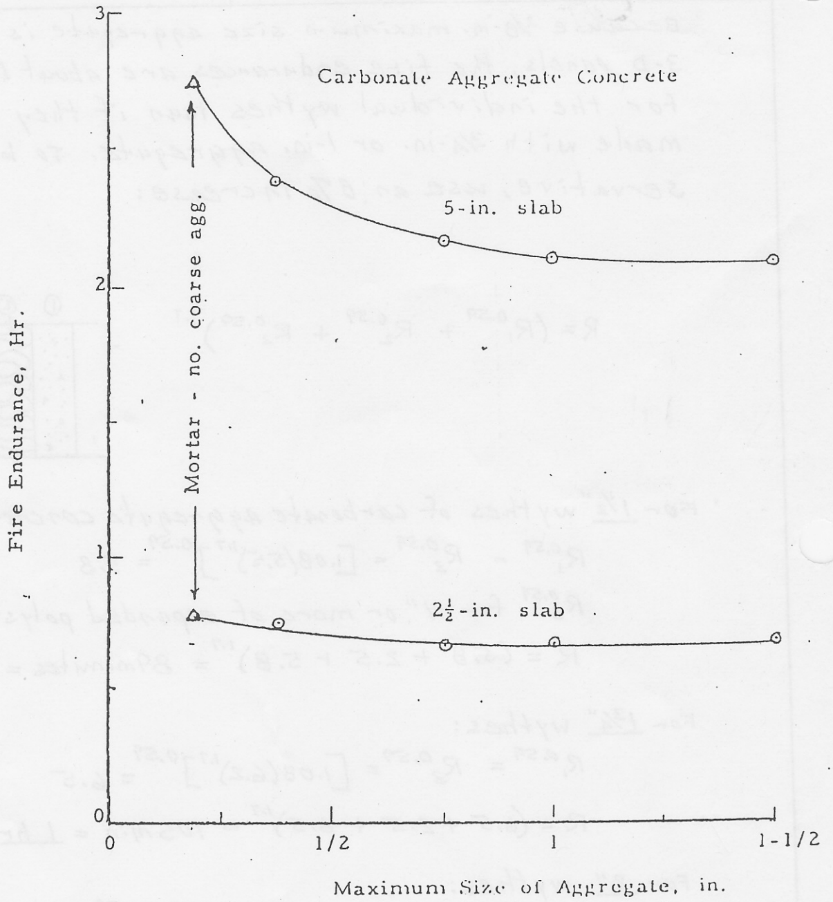
Fig. - Effect of Maximum Size of Aggregate on Fire Endurance
