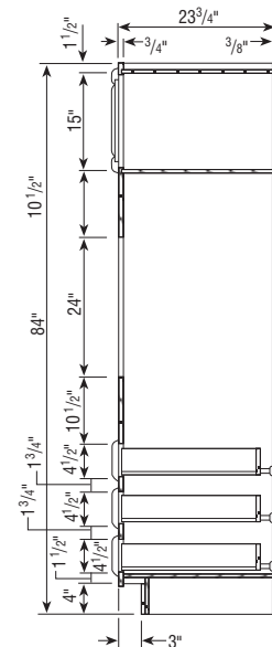
Single Oven Cabinet 1/4" Overlay Styles
