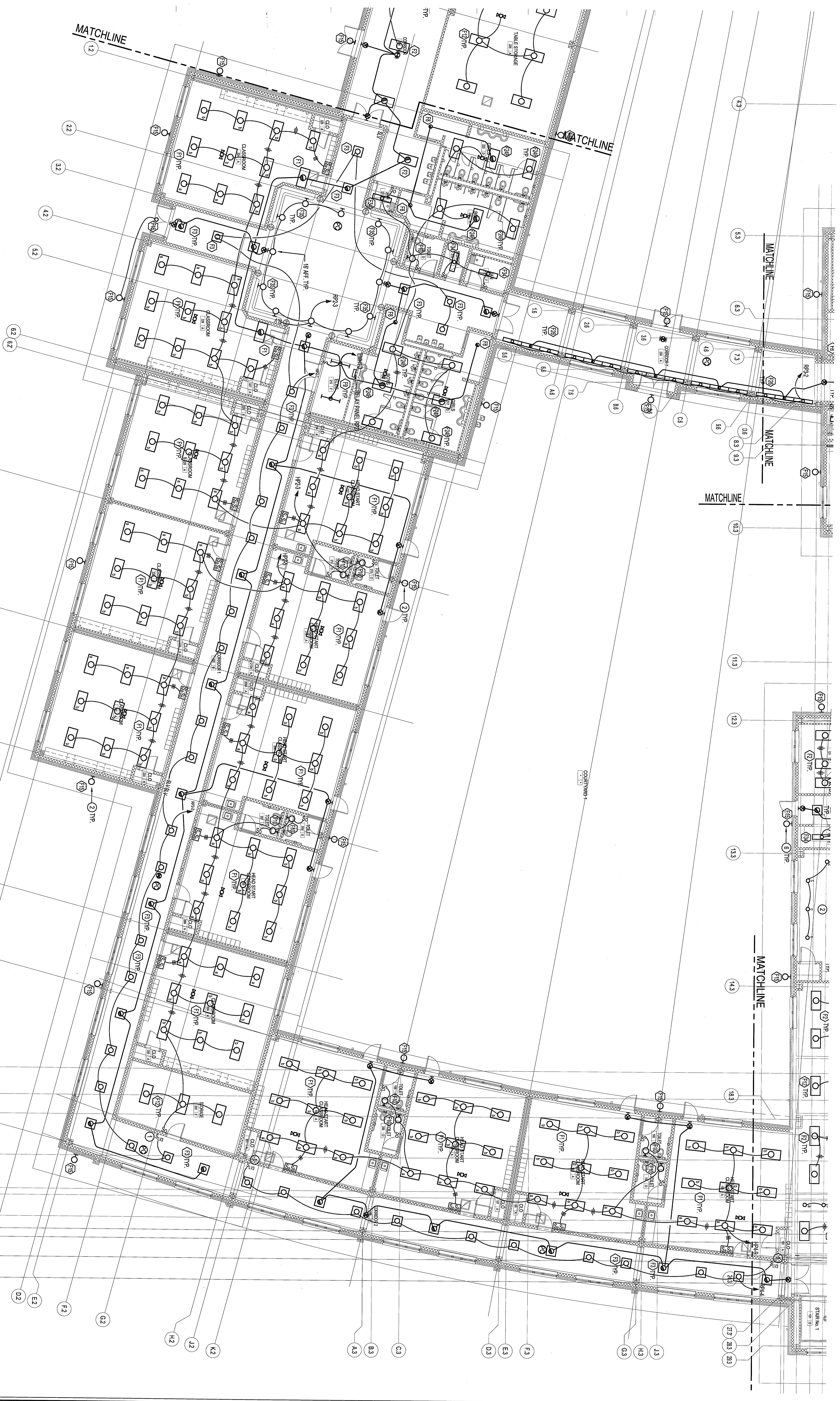
FIRST FLOOR PLAN - BLDG. 2 - LIGHTING SCALE: 1/8" = 1'-0"
