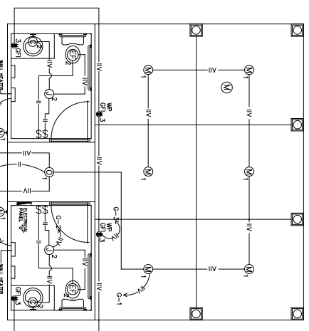
GAZEBO BLDG. LIGHTING & POWER SCALE: 1/4" = 1'-0"
