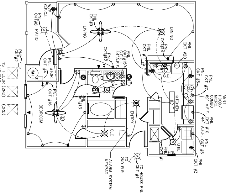
1 BEDROOM PLAN A 1ST FLOOR LIGHTING & POWER 1ST FLOOR SHOWN, 2ND & 3RD FLOORS SIMILAR SCALE: 1/4" = 1'-0"
