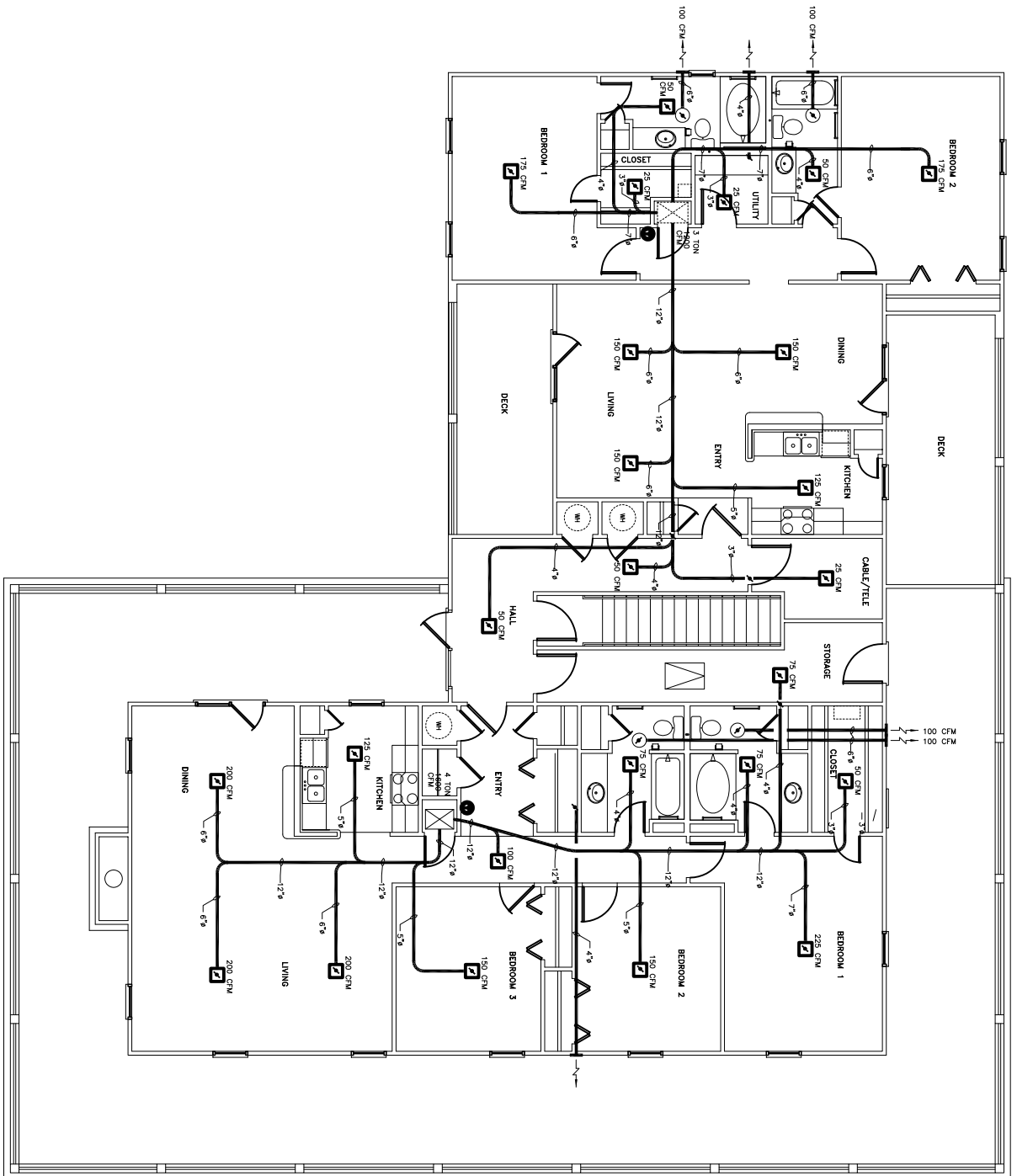
SECOND FLOOR LEASING OFFICE HVAC PLAN SCALE: 1/4" = 1'-0"
