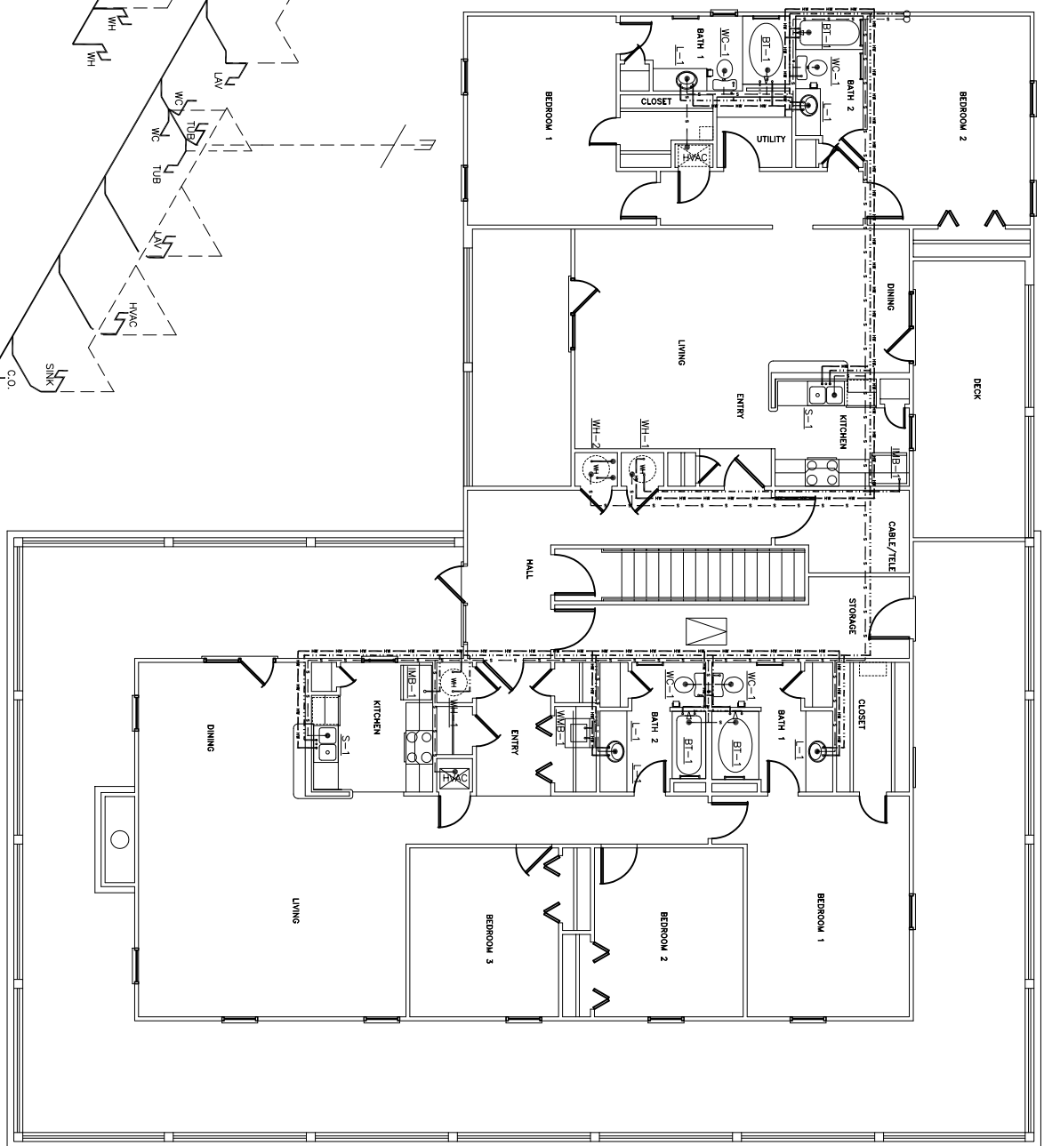
SECOND FLOOR LEASING OFFICE PLUMBING PLAN SCALE: 1/4" = 1'-0"
