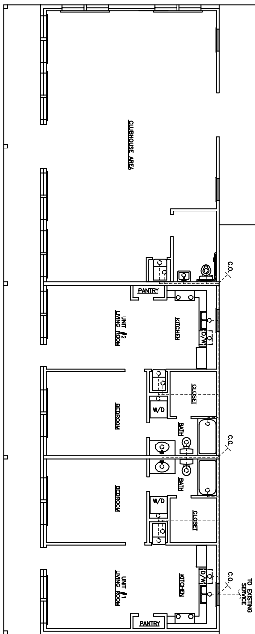
PLUMBING PLAN SCALE: 1/4"=1'-0"
