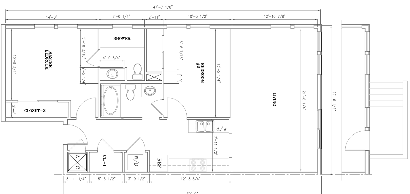
2 ENLARGED PLAN: UNIT #1 SCALE: 1/4"=1'-0"
