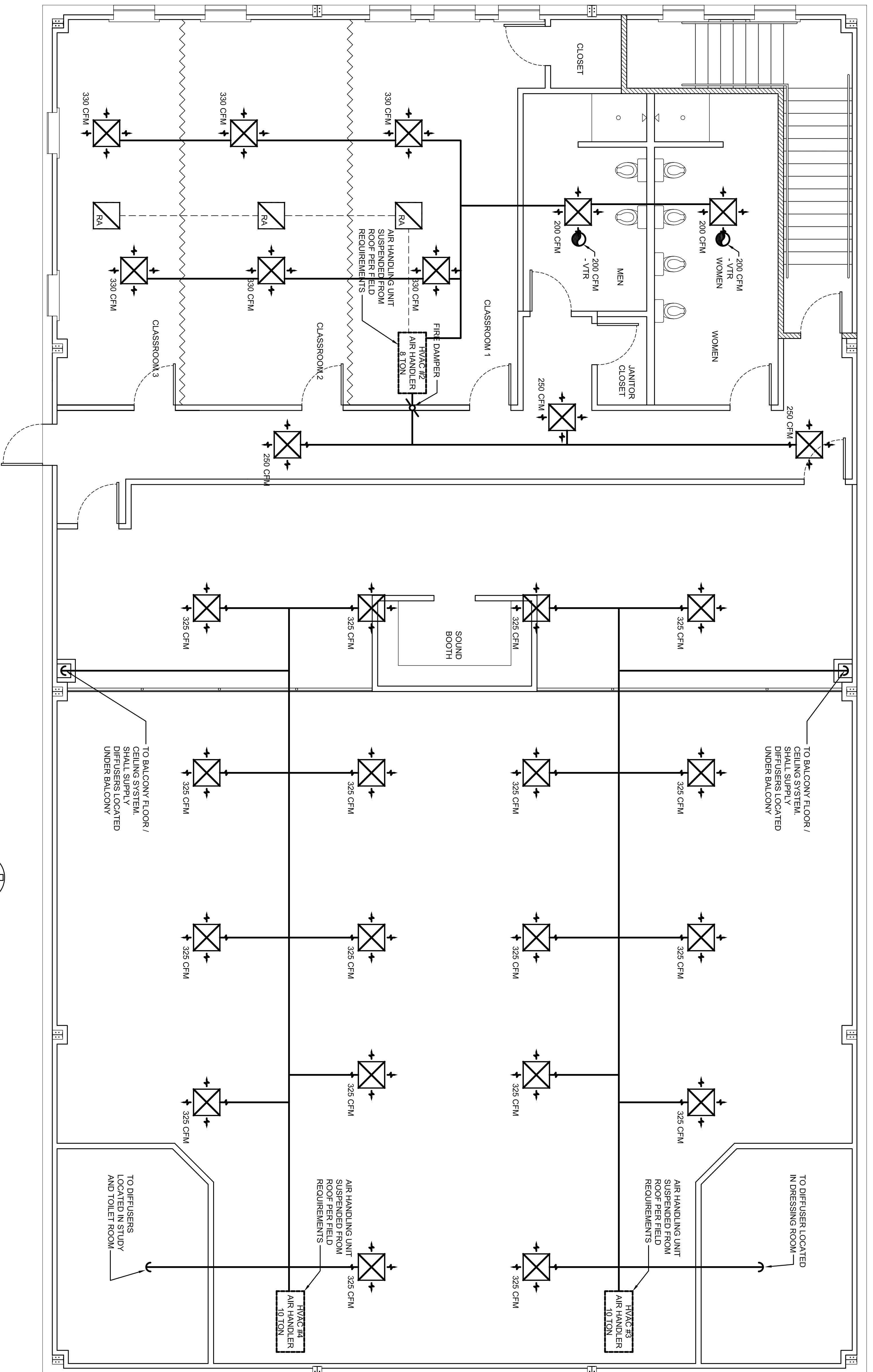
2nd FLOOR MECHANICAL PLAN SCALE: 1/4"=1'-0"
