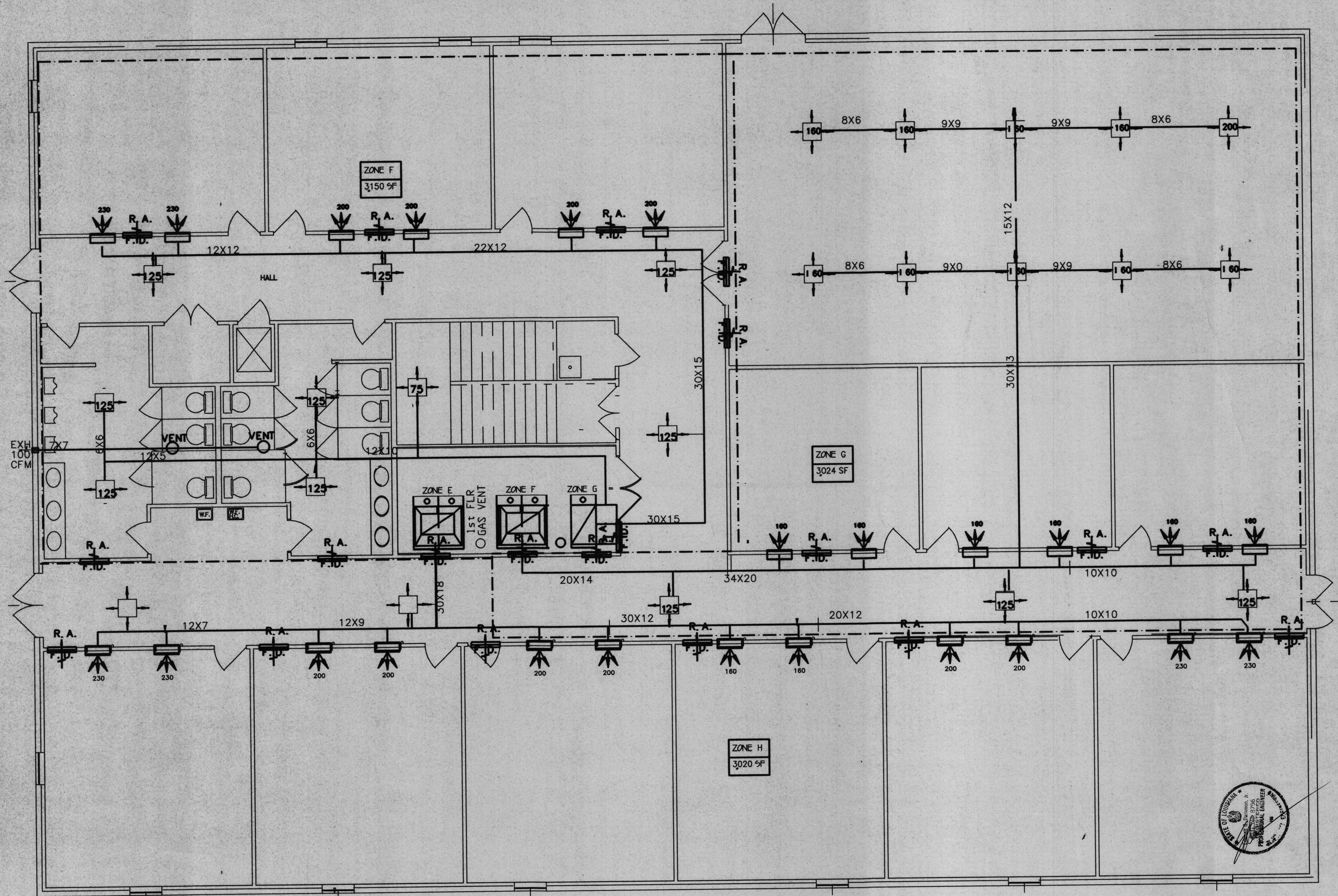
HVAC 2nd FLOOR PLAN
