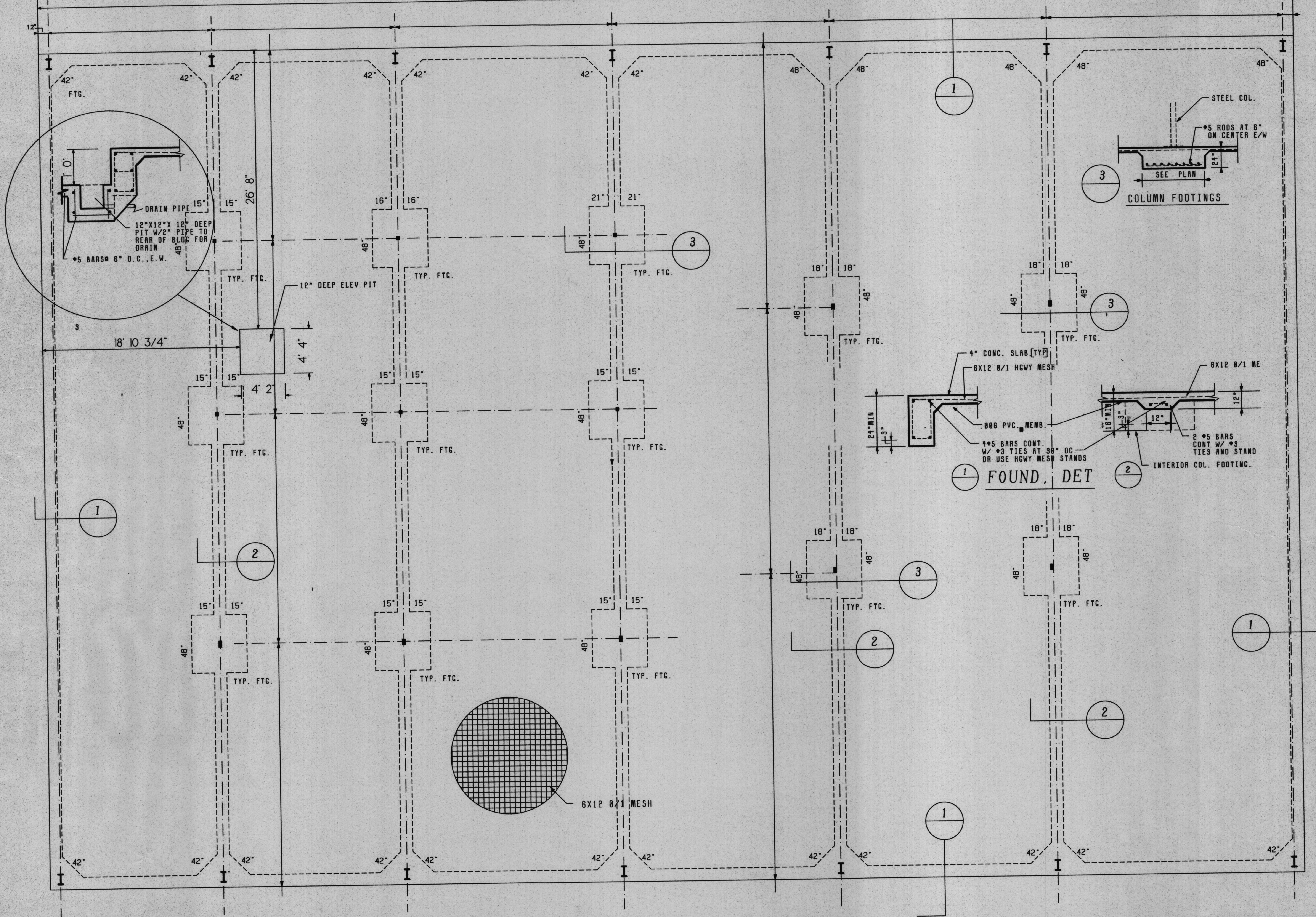
FOUNDATI ON PLAN
