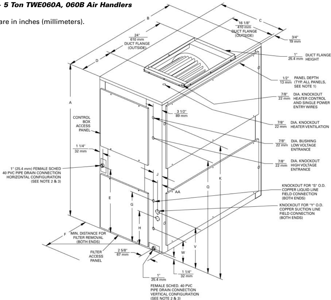
Figure DD-8 – 5 Ton TWE060A, 060B Air Handlers
