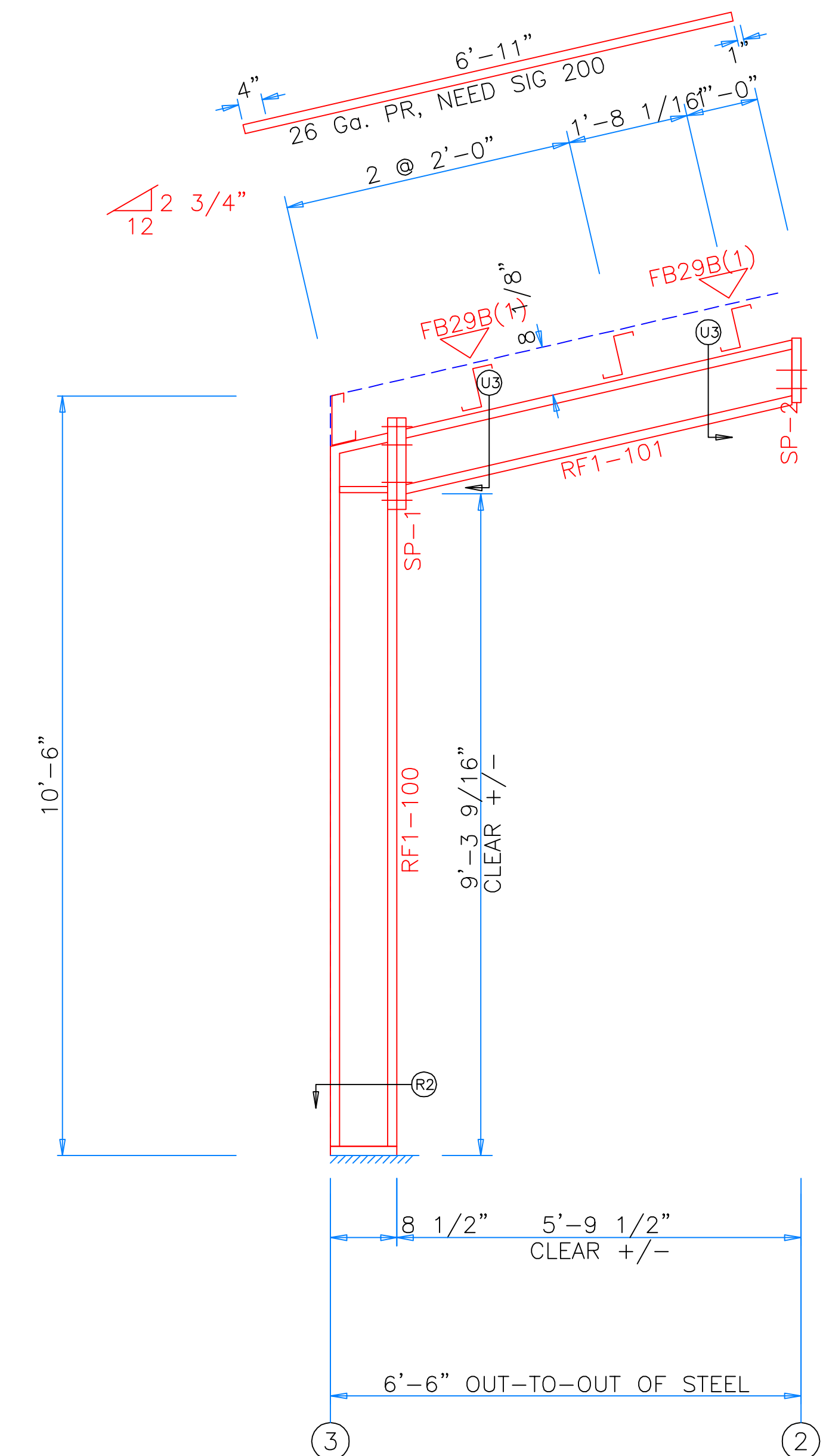
RIGID FRAME ELEVATION: FRAME LINE B C
