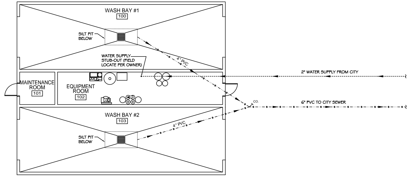
PLUMBING PLAN SCALE: 3/16"=1'
