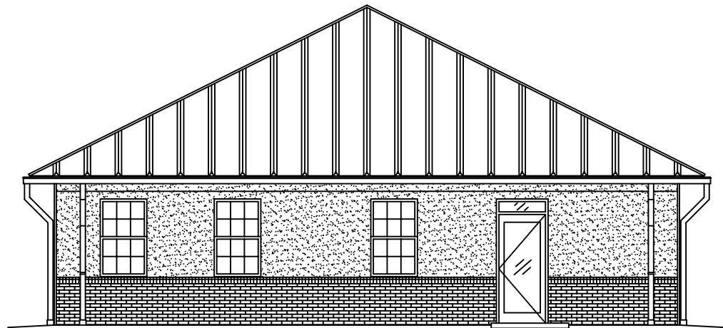
FRONT ELEVATION SCALE: 1/4"=1'
