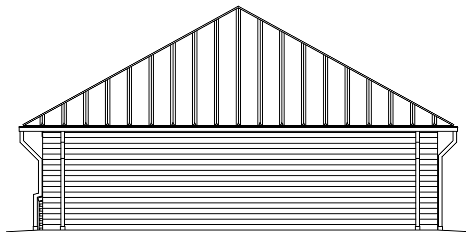
RIGHT SIDE ELEVATION SCALE: 1/4"=1'
