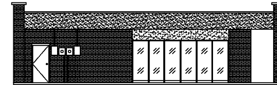
NEW SOUTH SIDE ELEVATION
