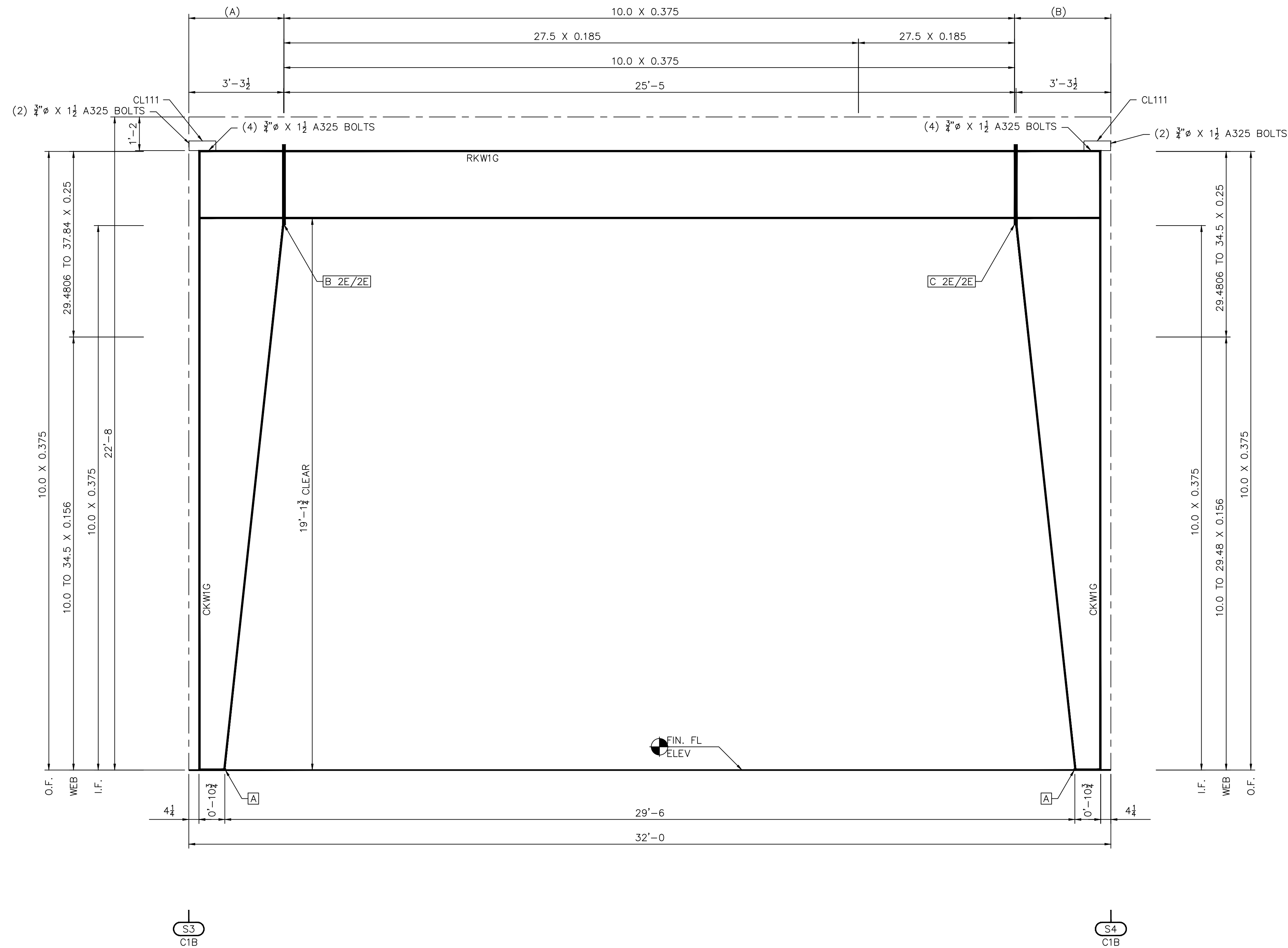
CROSS SECTION AT PORTAL FRAME
