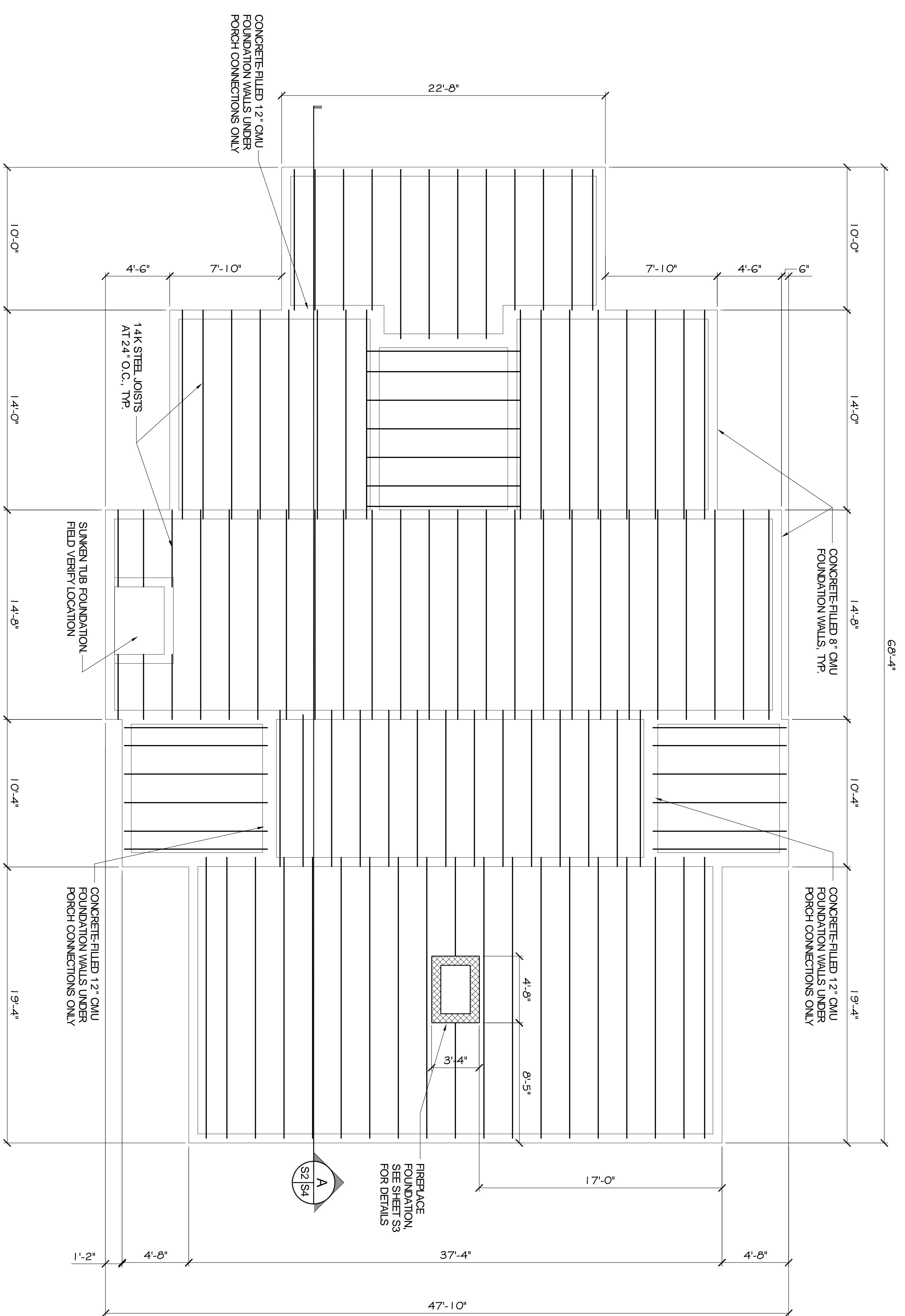
FLOOR LEVEL FOUNDATION FRAMING PLAN SCALE: 1/4" = 1'
