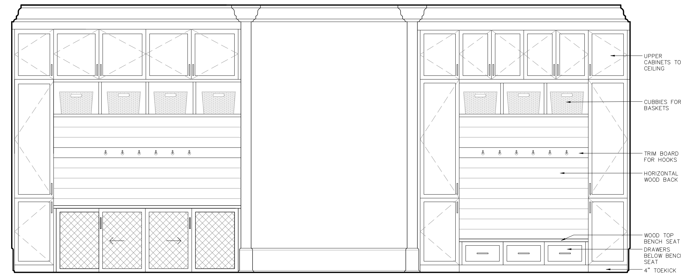
3 Breezeway / Dog Room Scale: 3/8" = 1'-0"
