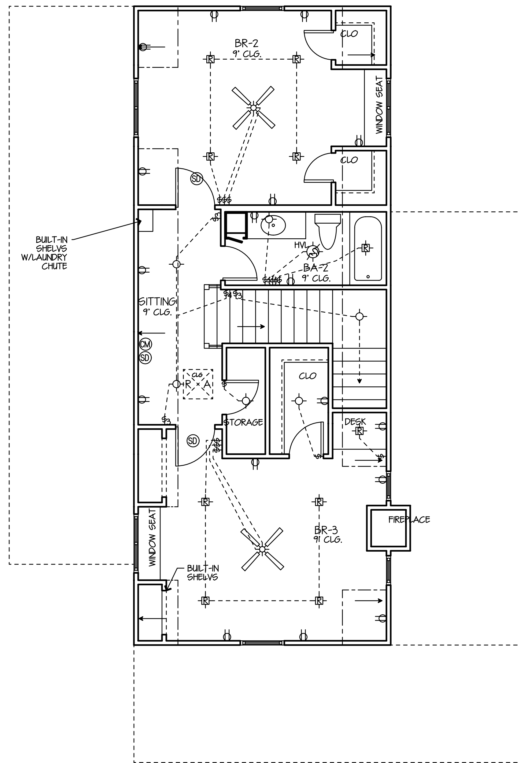
2ND LEVEL ELECTRICAL PLAN SCALE 1/4"=1'-0"
