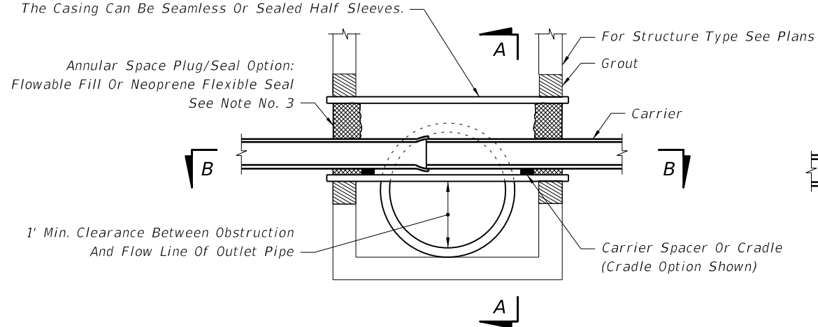
SECTION LONGITUDINAL TO CARRIER PIPE (Pressure Or Fluid Carrier Installations)
