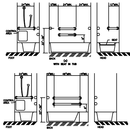
FIG. 32 GRAB BARS AT BATHTUBS N.T.S.
