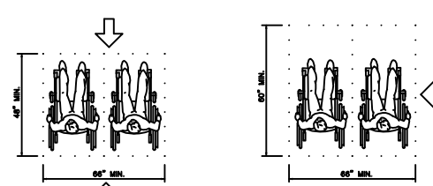
FIG. 46 SPACE REQUIREMENTS FOR WHEELCHAIR SEATING SPACES IN SERIES N.T.S.
