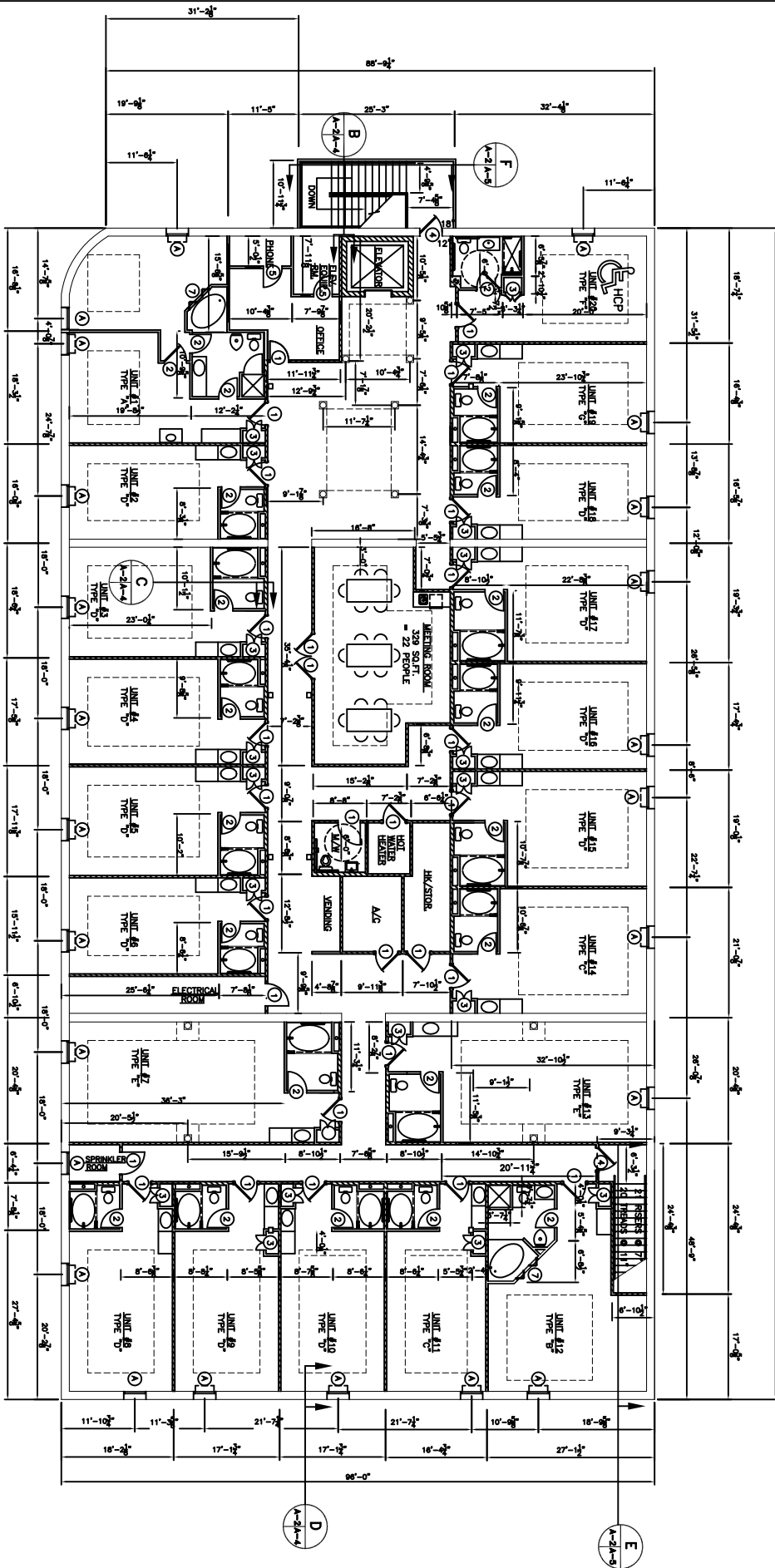
SECOND FLOOR PLAN SCALE: 1/8" = 1'-0"
