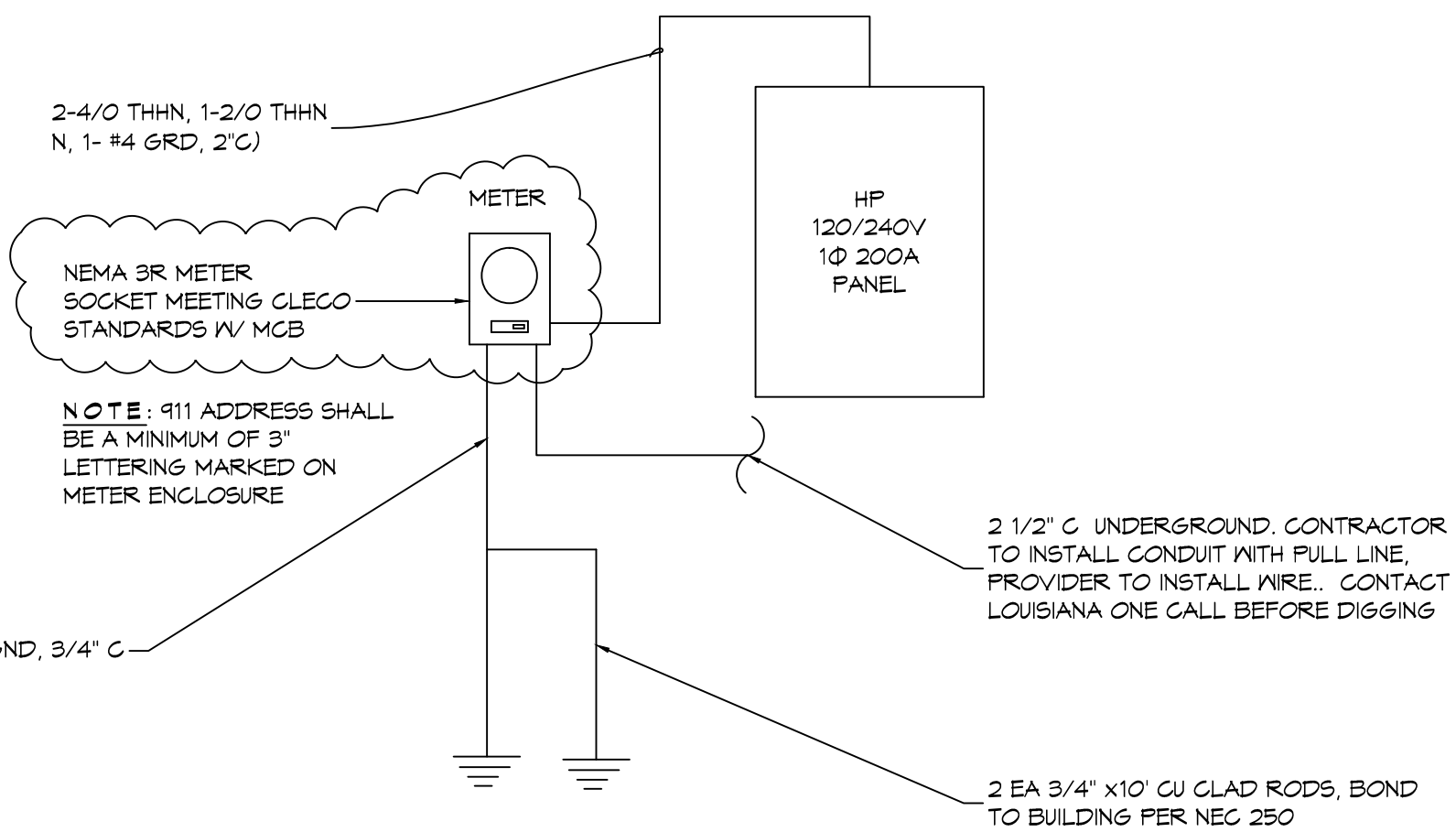
ONE-LINE DIAGRAM SCALE: NTS
