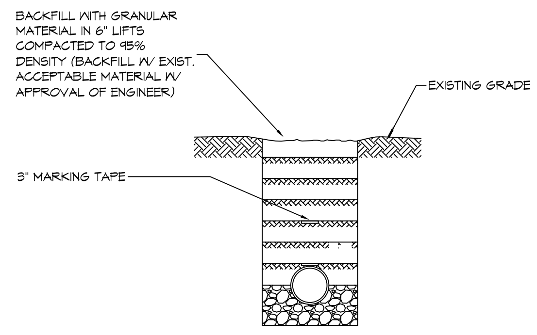
4 DETAIL SCALE: NTS ELECTRICAL SERVICE CONDUIT
