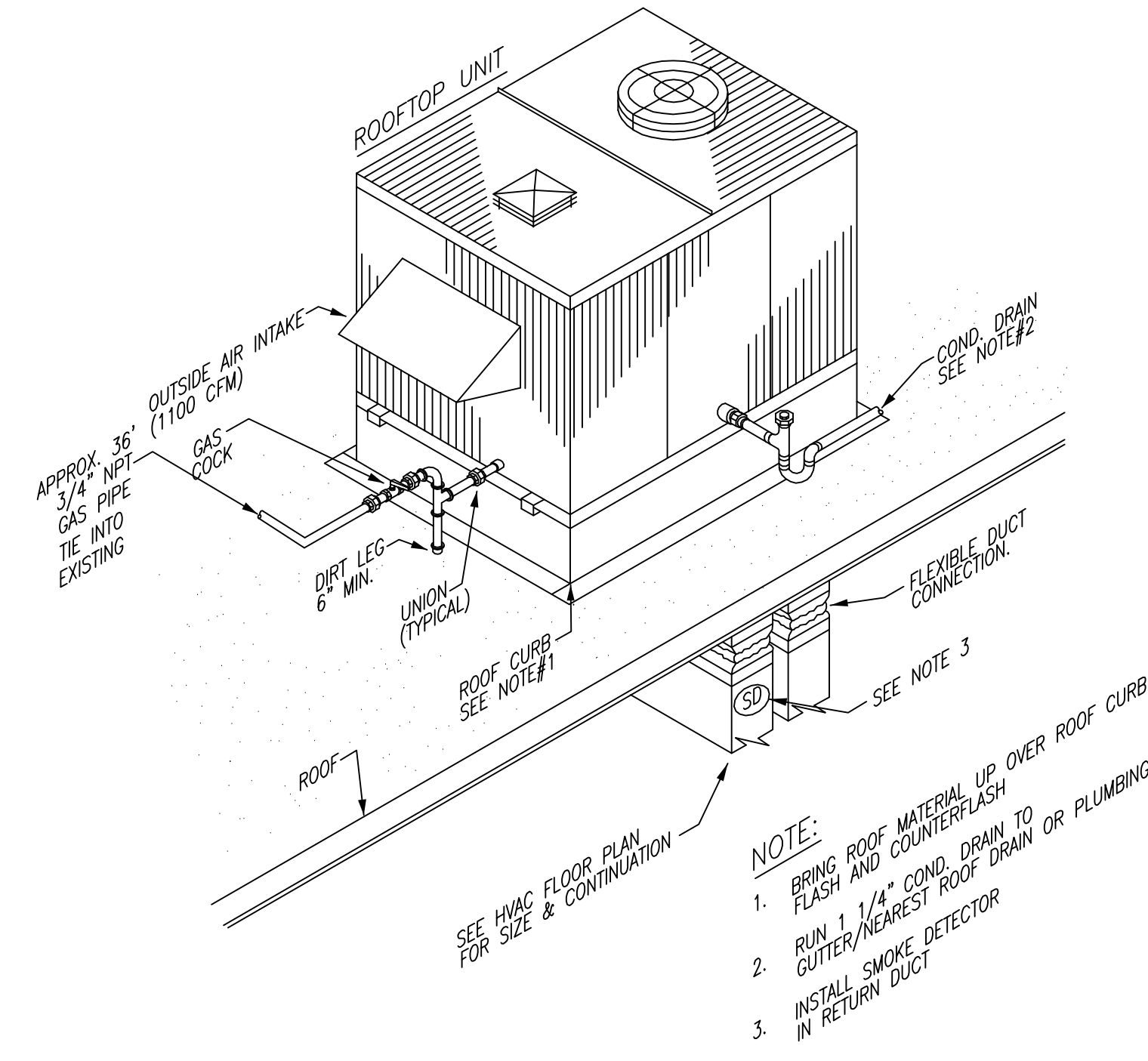
D TYPICAL ROOF TOP INSTALLATION AHU DETAIL
