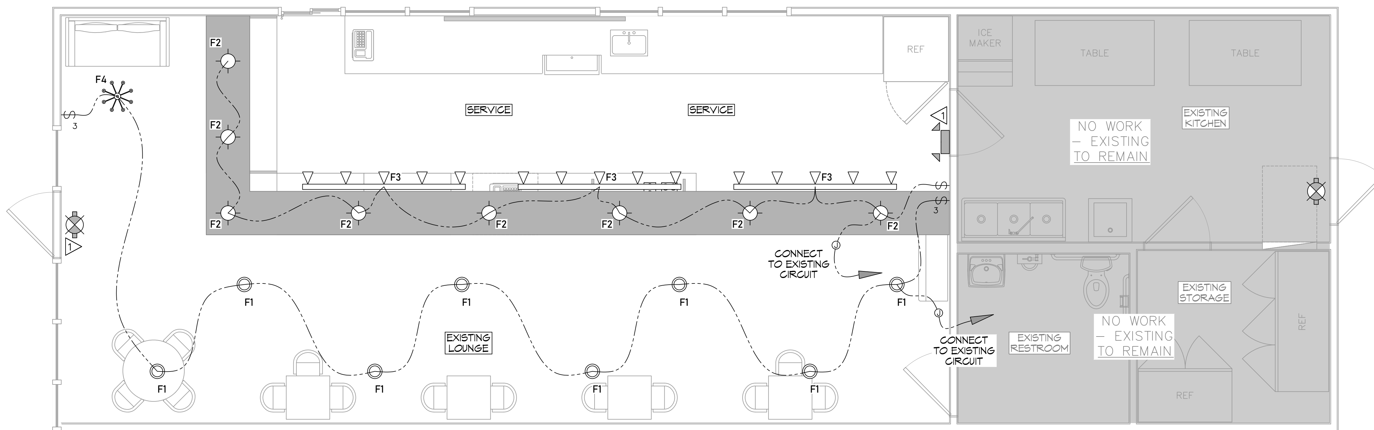
10 LIGHTING PLAN SCALE: 3/8"=1'-0"
