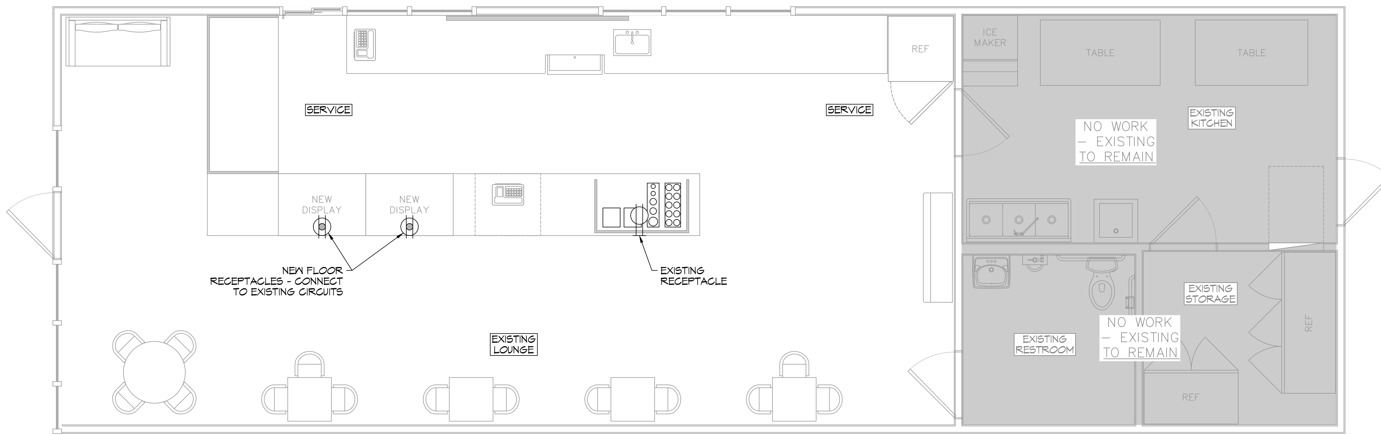
9 POWER PLAN SCALE: 3/8"=1'-0"
