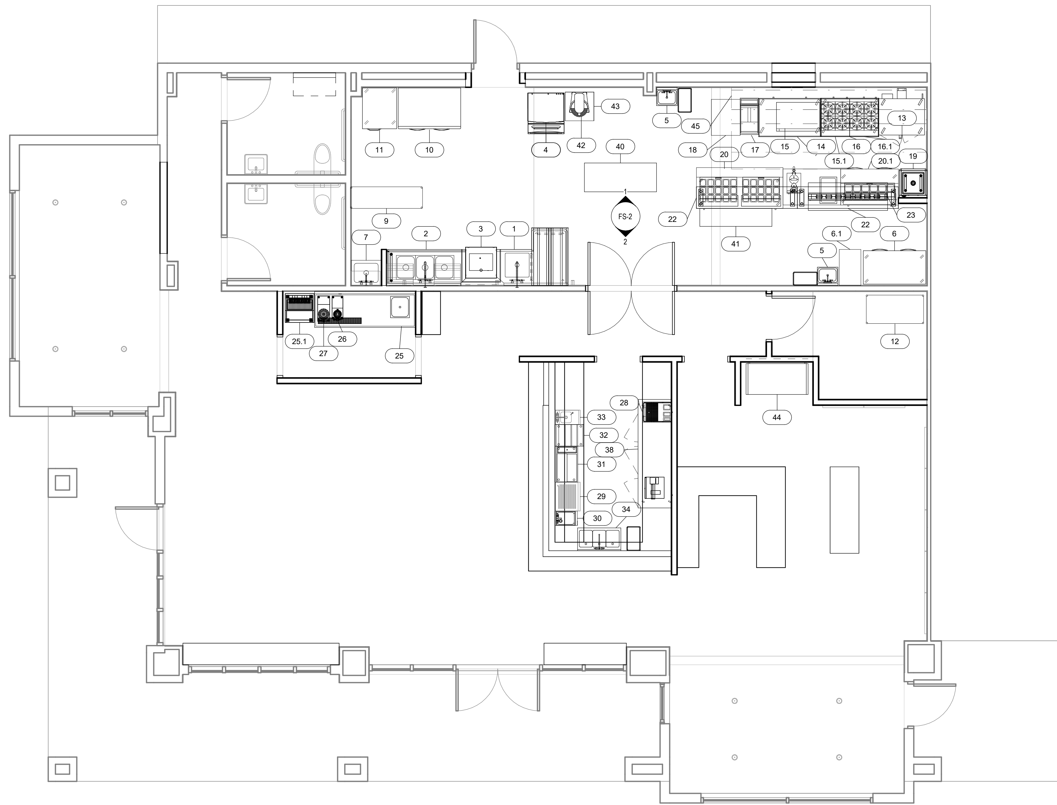
1 Foodservice Floor Plan FS-1 1/4" = 1'-0"
