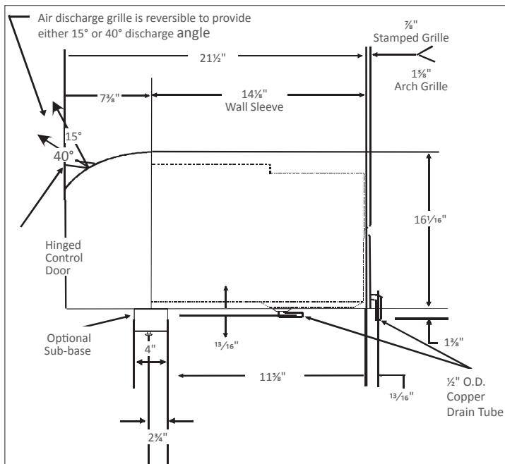
RIGHT VIEW
