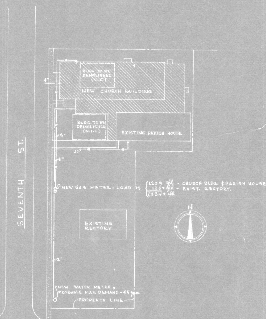
PLOT PLAN SCALE: 1" = 40'-0"
