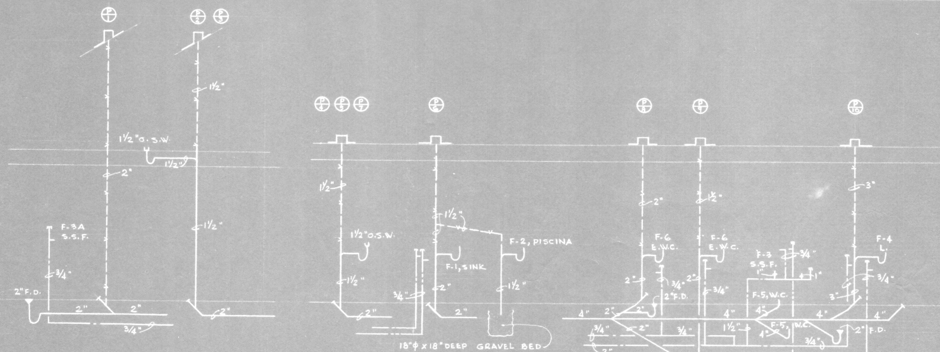
RISER DIAGRAM
