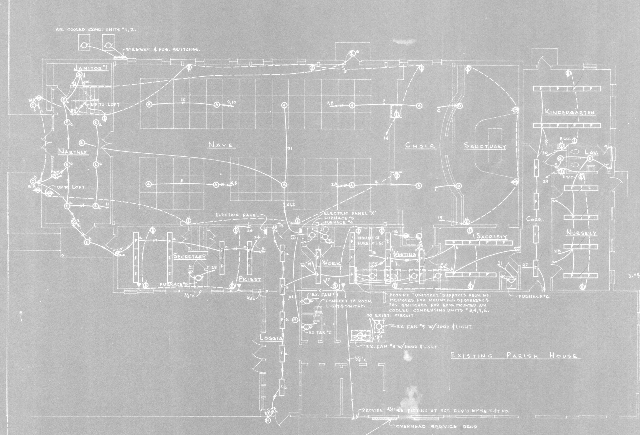
FLOOR PLAN - ELECTRICAL SCALE: 1/8" = 1'-0"
