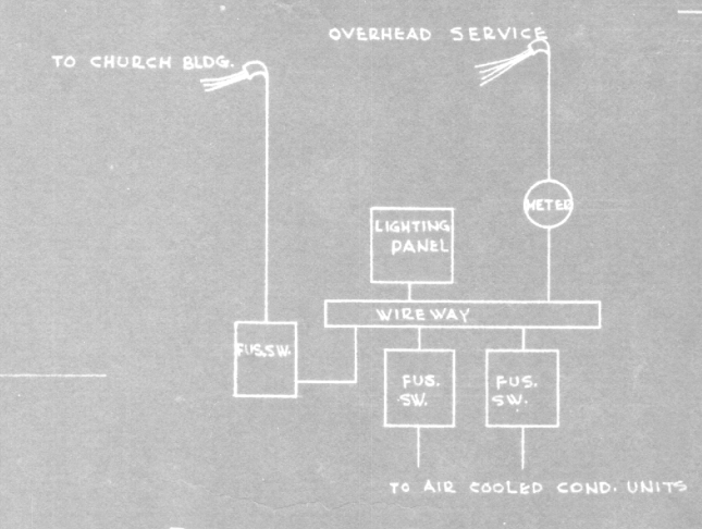
EXISTING SERVICE WIRING
