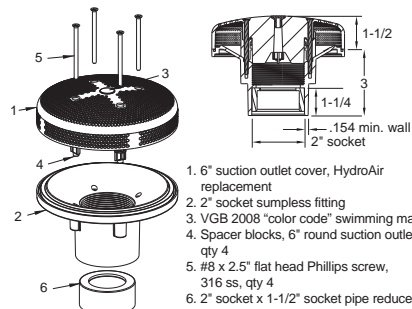
Part # 620T15Sxxx
