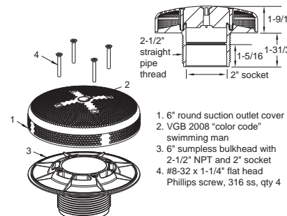
Part # 620SIxxx
