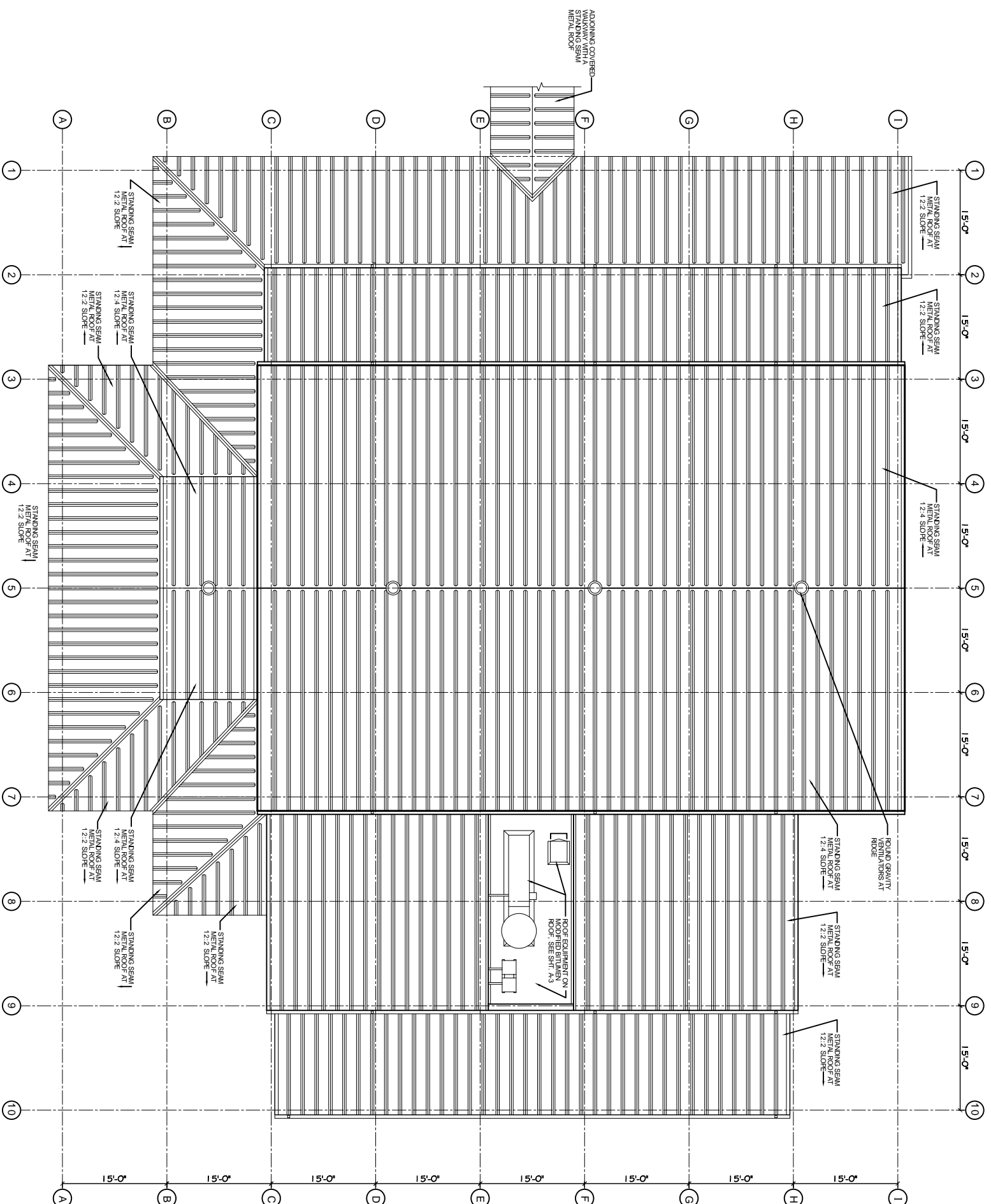
CAFETORIUM ROOF PLAN SCALE: 1/8" = 1'
