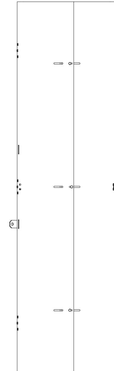
SLOT & HOLE COMBINATIONS USED FOR ADJUSTABILITY OF LADDER GUARD FOR DIFFERENT LADDER WIDTHS
