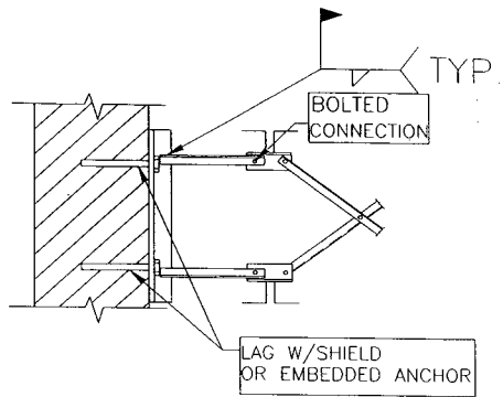
BOLTED DIAGONAL BRIDGING TERMINUS AT WALL
