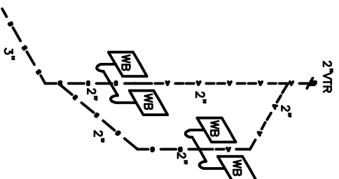
R9 RISER DIAGRAM
