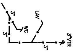
R1 RISER DIAGRAM
