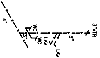
R9 RISER DIAGRAM
