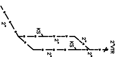
R13 RISER DIAGRAM
