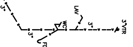
R19 RISER DIAGRAM
