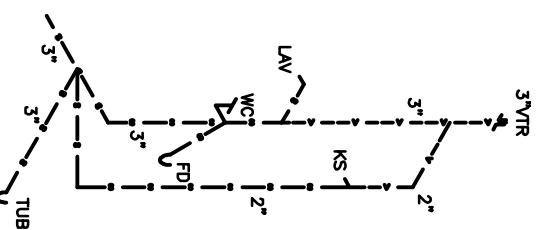
R18 RISER DIAGRAM
