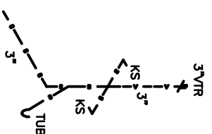
R3 RISER DIAGRAM
