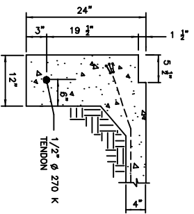
SECTION (AT EXT. W/O BRICK)
