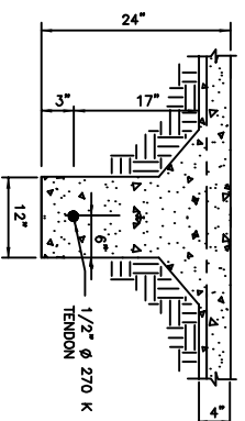
SECTION (AT INTERIOR BEAMS)
