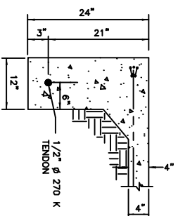
SECTION (AT EXT. W/O BRICK)
