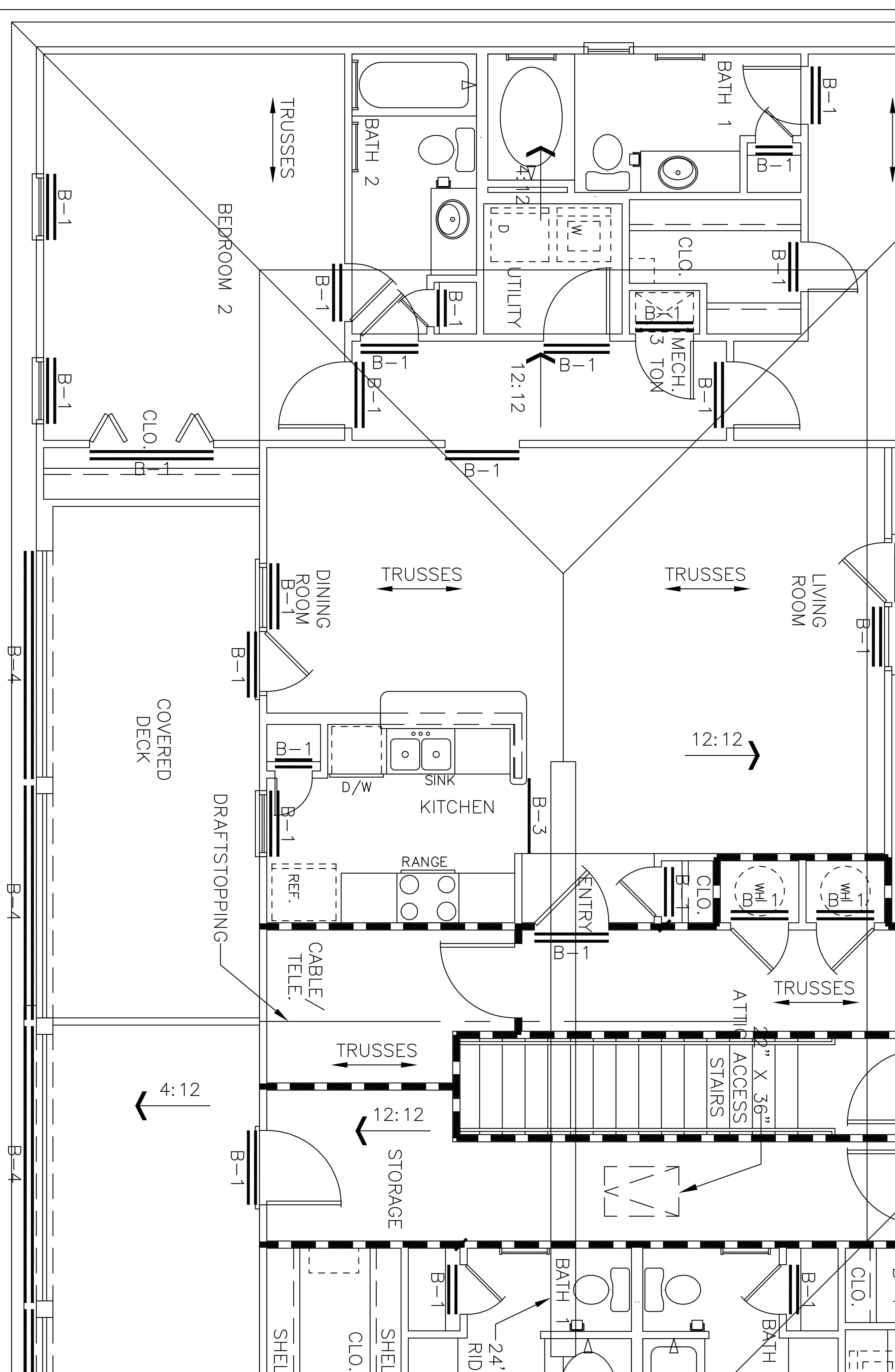
SECOND FLOOR LEASING OFFICE FRAMIN SCALE: 1/4" = 1'-0"
