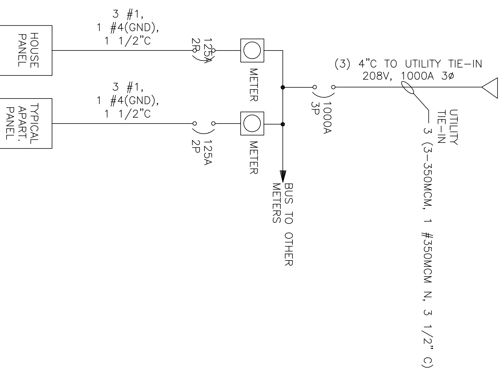
TYPICAL APARTMENT ONE LINE DIAGRAM
