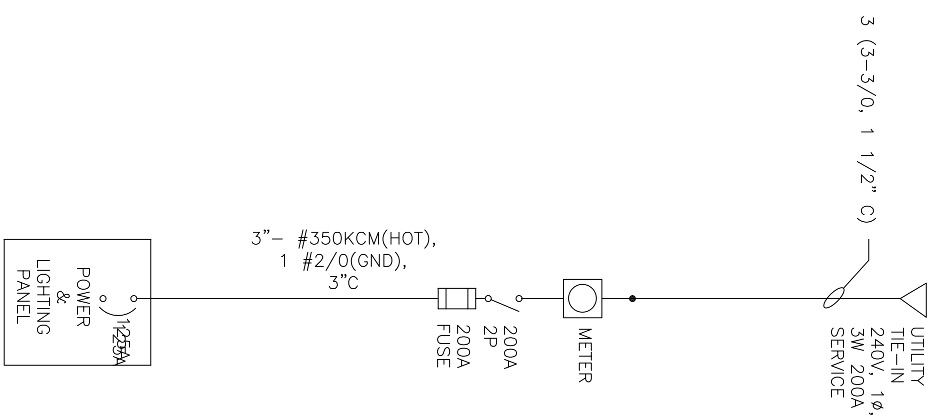
ONE LINE DIAGRAM - LEASING OFFICE
